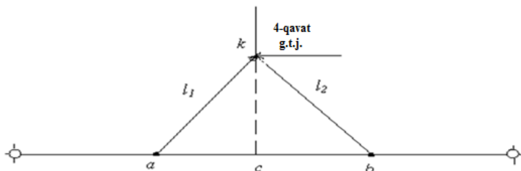
6.3-rasm. Chiziqli kestirma usuli
