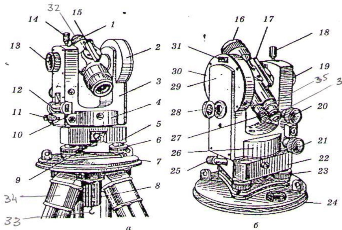
4.2-rasm. T30 teodolit tuzilishi
