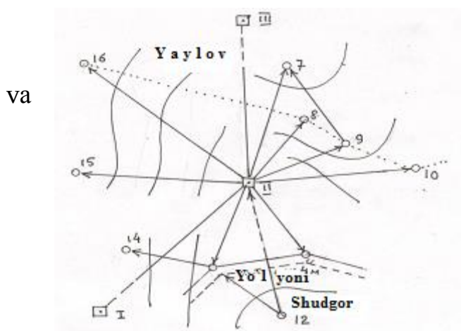
6.14-rasm. Taxeometrik syomka abrisi
