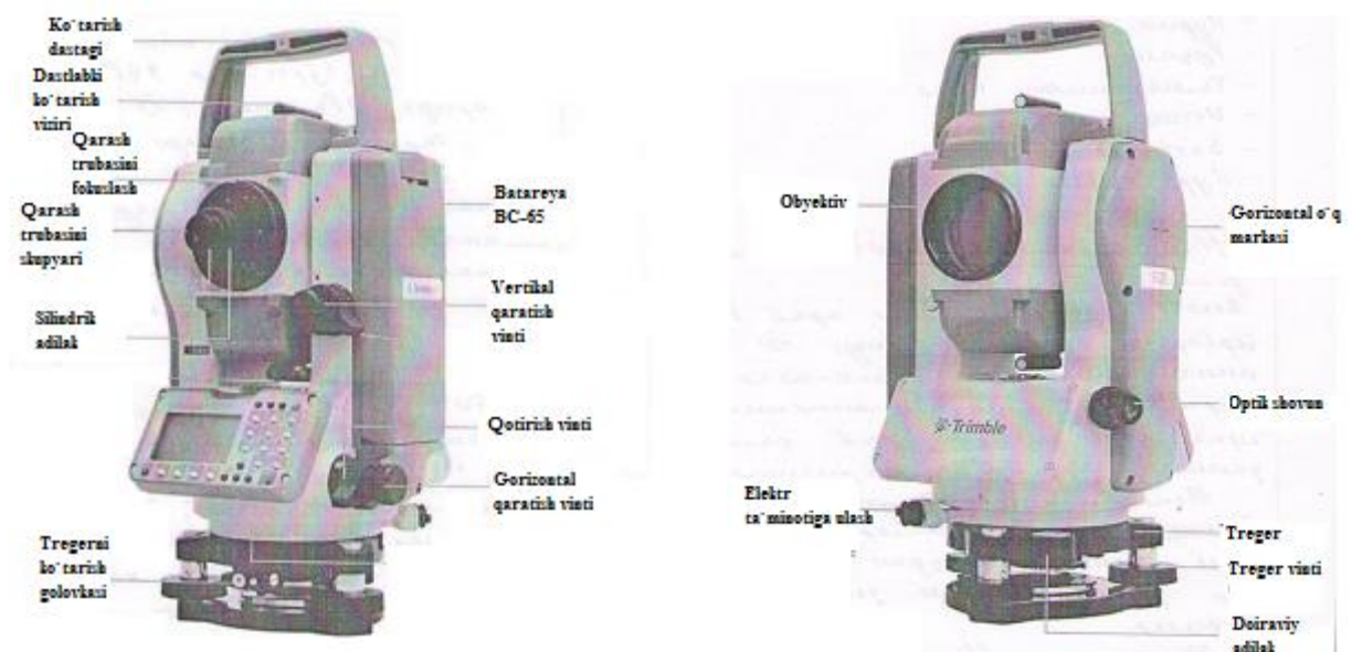
6.13-rasm. Elektron taxeometr
