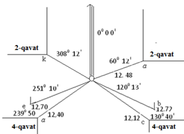
6.1-rasm. Qutbiy usulda planga olish
