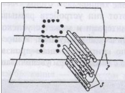
22.11-rasm. Mozaikali (matrisiali) printyerning ishlash prinsipi
