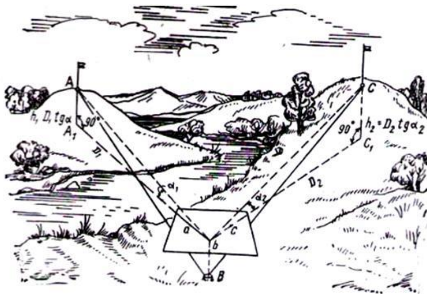
6.16-rasm. Grafik usulda plan olish
