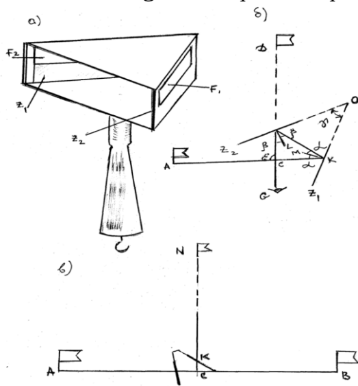
4.4-rasm. Ekker va undan foydalanish
