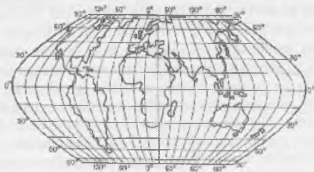
15-rasm. Pseudosilindrik proyeksiya
