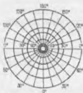
14-rasm. Normal azimutal proyeksiya
