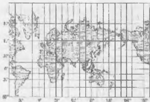
13-rasm. Normal silindrik proyeksiya
