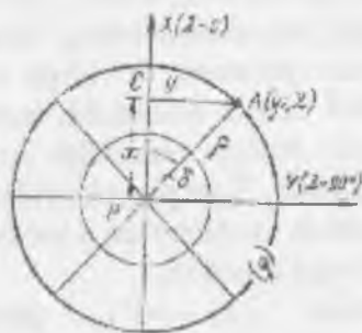
26-rasm. Normal azimutal proyeksiya koordinatalari tizimi
