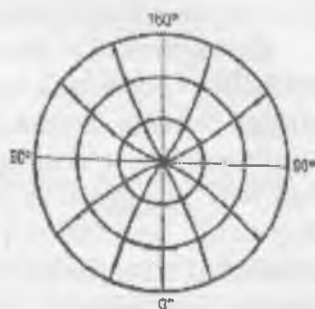
17-rasm. Normal psevdoozimal proyeksiya
