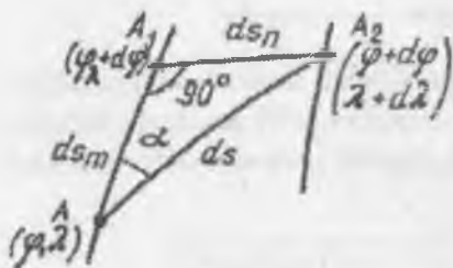
5-rasm. Elementar sferoidik uchburchak
