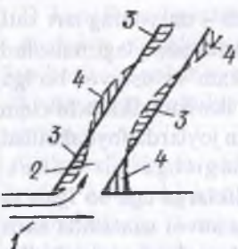
7.33-rasm. Suv olish kallaklarini daryo oqimi o'nalishi bo'yicha siljishi: 1-daryo, 2-kanal, 3-loyqa to'planish zonasi; 4-yuvilish zonasi
