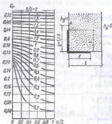
3.50-rasm. Q_r = f(S/l, c/l) funksiya grafiqi; S/l > 2 bo'lganda sarf
