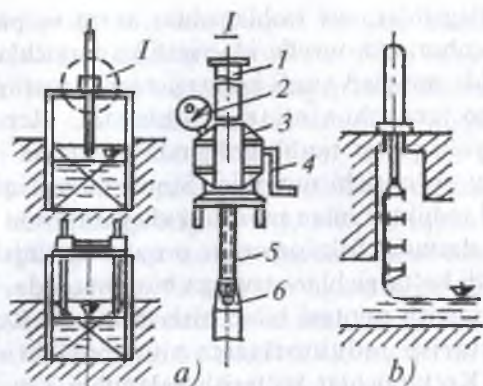
6.37-rasm. Qattiq tortqichli ko'tarish mexanizmlari:
