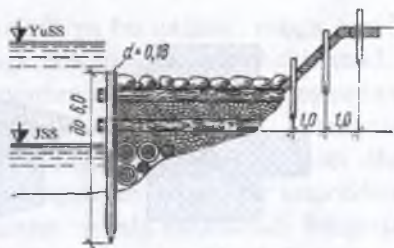
7.21-rasm. Fashina-tosh bilan mustahkamlash.
