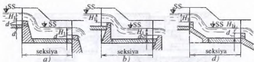
5.28-rasm. Sharshara tushish devorlari:
