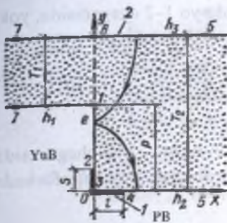
3.42-rasm. Yakka diafragmali yon devorda aylanma filtratsiya hisobi sxemasi: 1-to'g'on; 2-to'yinish konturi.
