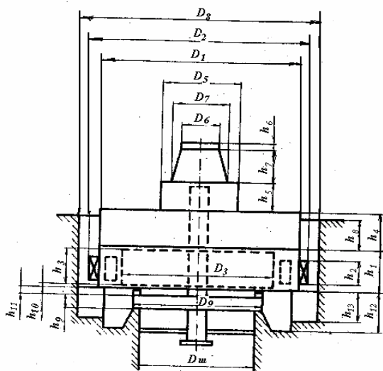
12 – rasm.Osma turdagi gidrogenerator
