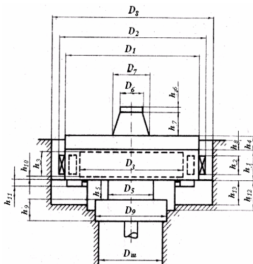
10-rasm. Podpyatniki turbinaning pastki krestovinasiga tiralgan zontli gidrogenerator
