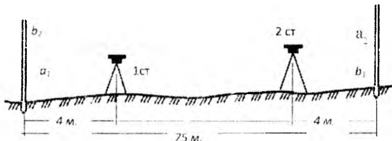
11.14-shakl. Qarash trubasining vizir o'qi silindrik adilak o'qiga parallel bo'lish shartini tekshirish sxemasi
