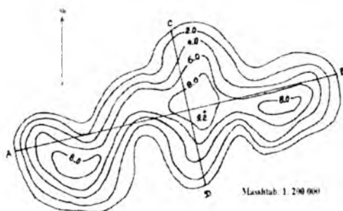
4.2-rasm. Kumushko'lning izobatlarda ifodalangan plani
