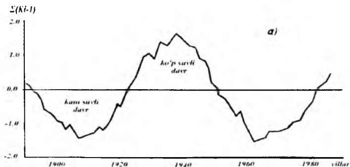
1.10.2-rasm. Daryo oqimining yig'indi (a) egri chizig'i.
