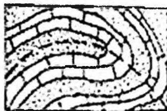
37-rasm. To'ngarilgan burma.
