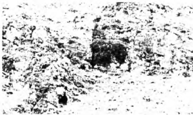
62-rasm. Otyaylov tog' yon bag'ridagi g'or.
