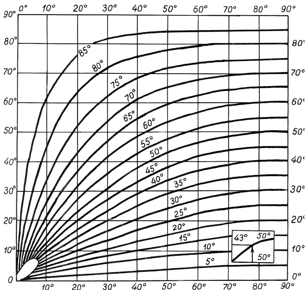
9-rasm. Qatlam yo'nalishiga perpendikular bo'lmagan chiziqda uning yotish burchagini aniqlash uchun nomogramma
