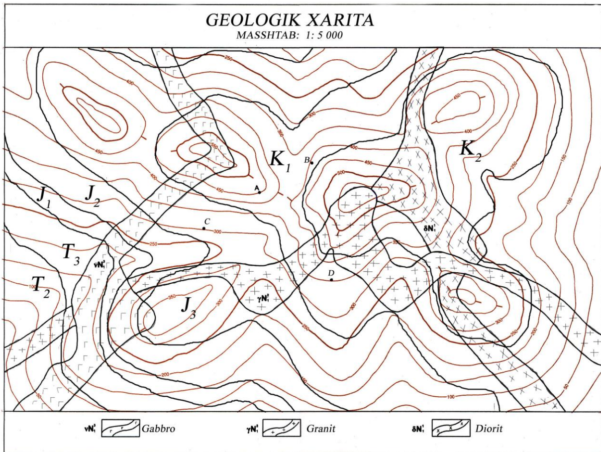
7-rasm. Geologik xarita
