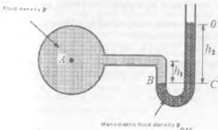
2.26.7-rasm. "U" -Trubkali manometr
