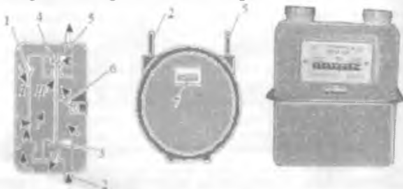
2.26.13-rasm. GKF tipidagi diafragma hisoblagich
