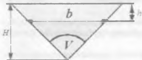
3.21.3-rasm. Veyr V chuqurligi
