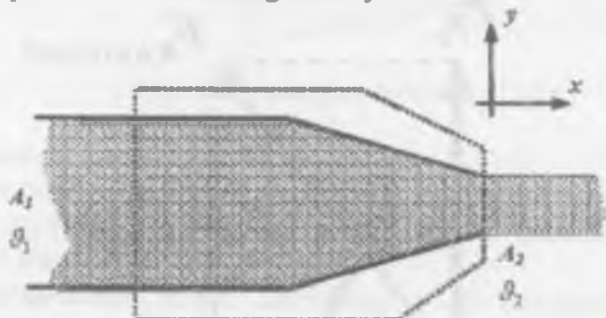
3.25.4-rasm. Quvur soplodagi kuchlar
