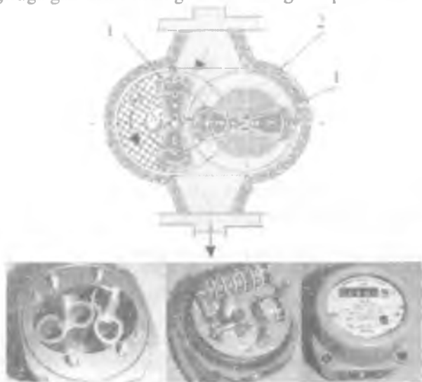
2.26.14-rasm. Rotatsion hisoblagich
