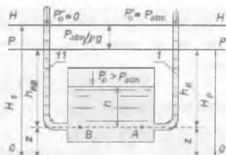
2.33.2-rasm. Naporni aniqlash
