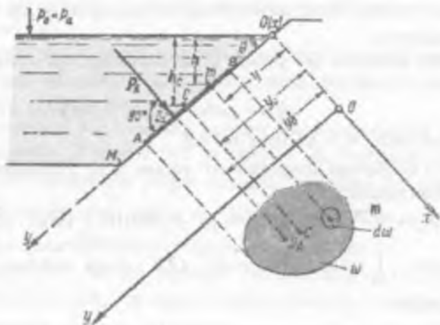
2.34.1-rasm. Bosim markazini aniqlash
