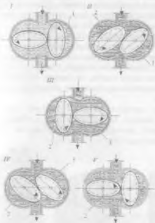
2.26. 12-rasm. Ovalsimon shesternyali hisoblagich sxemasi
