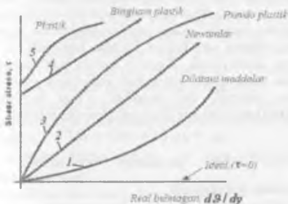
2.17.2-rasm. Siljish deformatsiyasi tezligiga bog'liq siljish d\gamma/dt
