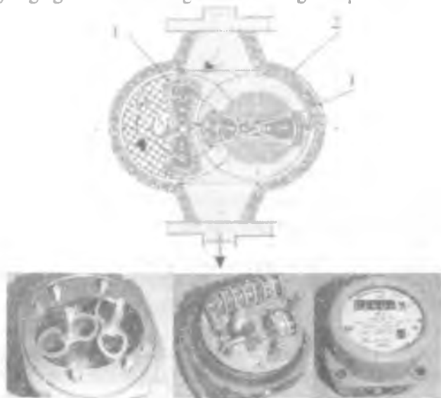
2.26.14-rasm. Rotatsion hisoblagich
