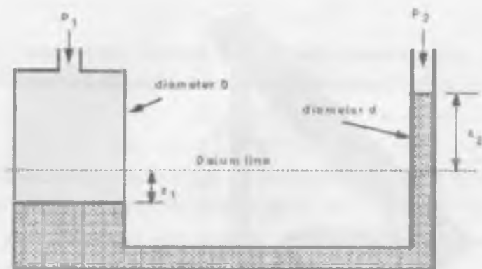
2.26.9-rasm. Quvurlik "U" simon manometriga o'tish
