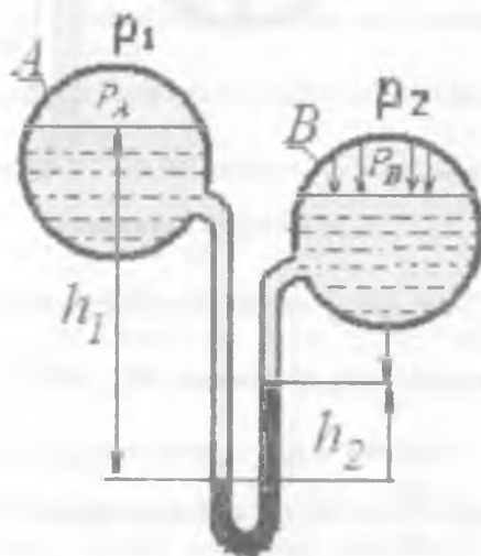
2.26.3-rasm. Differentsial manometr
