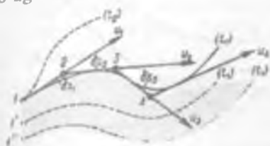
3.2.5-rasn. Beqaror harakatdagi oqim chizig'i.
