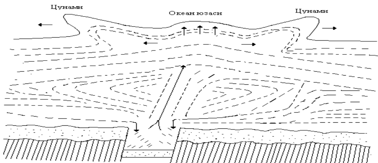
4.3-rasm. Sunamining hosil bo'lishi
