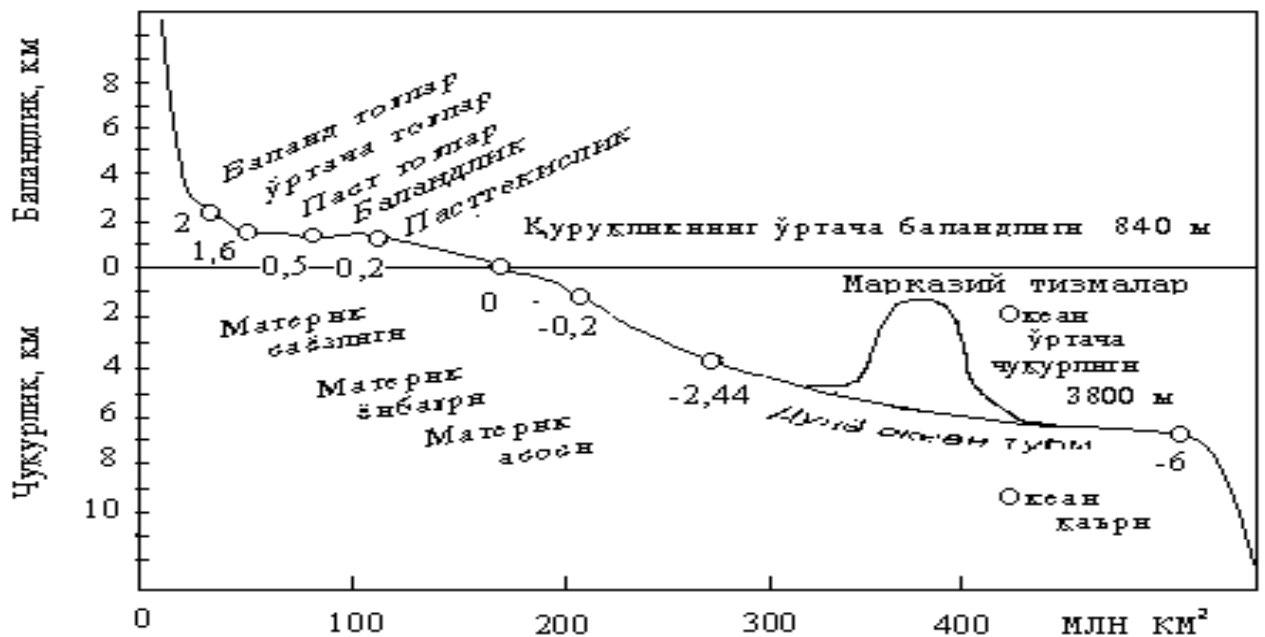
2.3-rasm. Gipsografik egri chiziq
