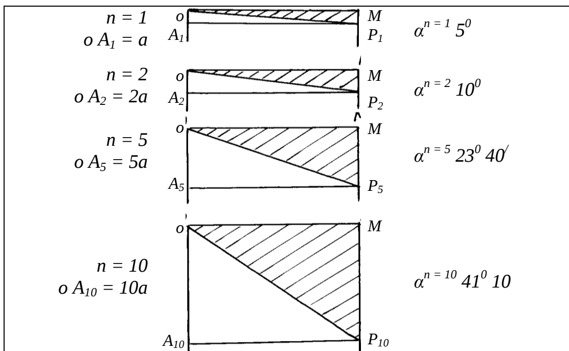
13.3-rasm. Vertikal miqyosning gorizonta miqyosga nisbatan oshirilganida qatlam yotish burchagi va qalinligining o'zgarishi
