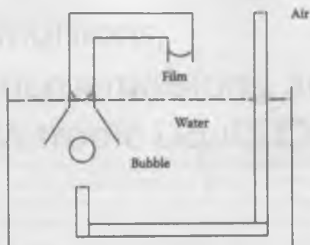
FIGURE 8.6 Bubble foam separation method for wastewater purification.
