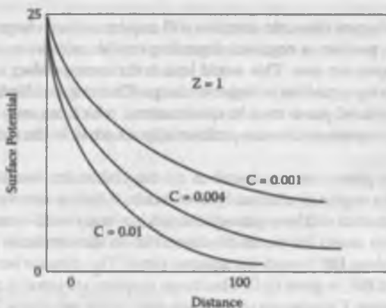
FIGURE 4.9 Double-layer model (variation of \psi with distance).
