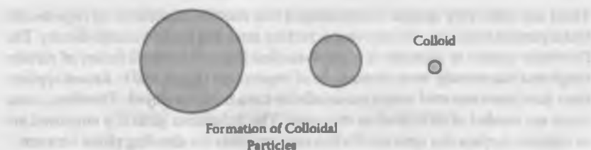
FIGURE 1.5 Formation of fine (colloidal) particles (schematic; size less than micrometer).
