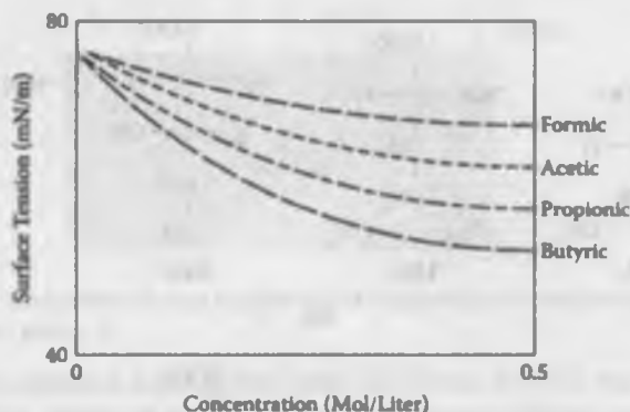
FIGURE 3.3 Surface tension data of a homologous series of short-chain acids in water.
