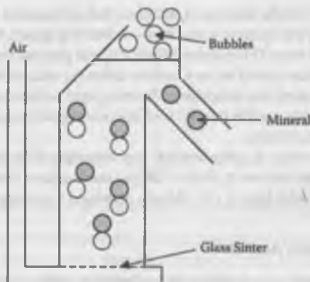
FIGURE 8.5 Apparatus used for froth flotation experiments.
