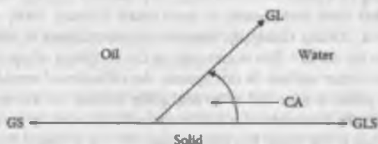
FIGURE 5.3 Contact angle at water–Teflon–octane interface.
