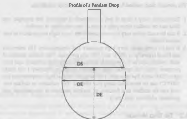
FIGURE 2.11 Pendant drop of liquid (shape analysis).
