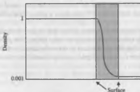
FIGURE 2.1 Change of density of a fluid (water) near the surface.
