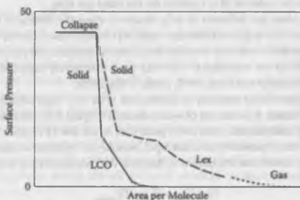
FIGURE 4.6 \Pi versus A isotherms for different types of states: (a) gas film; (b) liquid-expanded ( L_{ex} ) and liquid-condensed ( L_{co} ); solid films; collapse state.
