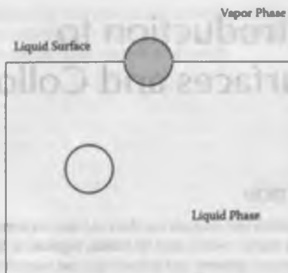
FIGURE 1.1 Surface molecules (schematic).
