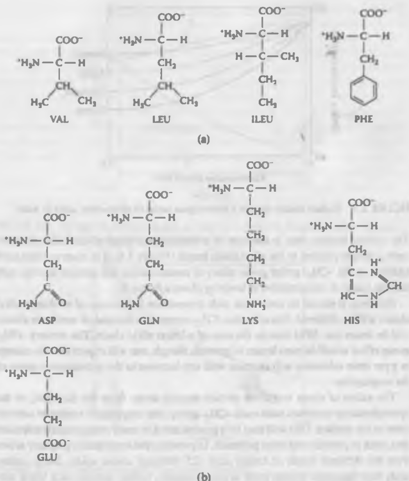
FIGURE 3.4 Polar (a) and apolar (b) amino acids.
