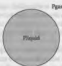
FIGURE 2.5 Liquid drop and \Delta P ( = P_{\text{LIQUID}} - P_{\text{GAS}} ) (at a curved liquid-gas interface).
