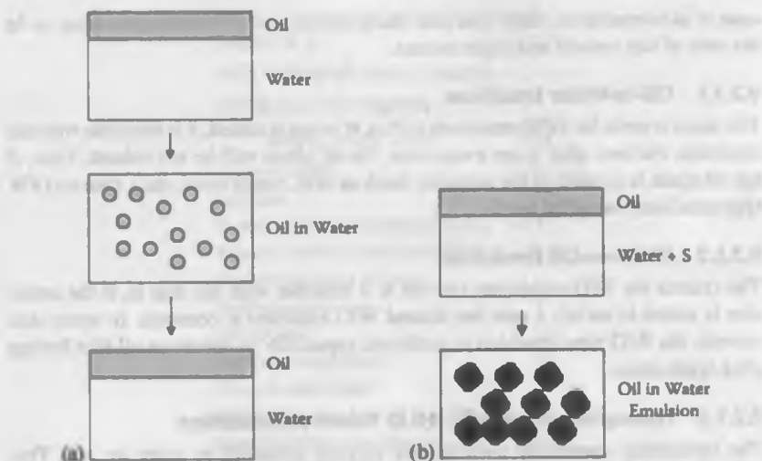
FIGURE 9.1 Mixing of oil and water (a) or oil and water + surfactant (b) by shaking.
