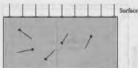
FIGURE 3.5 Orientation of soap (surface-active substance) at the surface of water (alkyl group:—, polar group: \rightarrow ).
