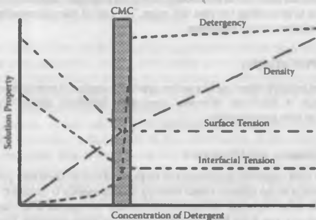
FIGURE 3.20 Change in detergent solution properties as related to CMC (schematic).
