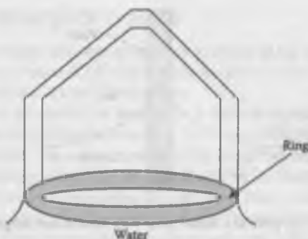
FIGURE 2.12 Ring method (see text for details).
