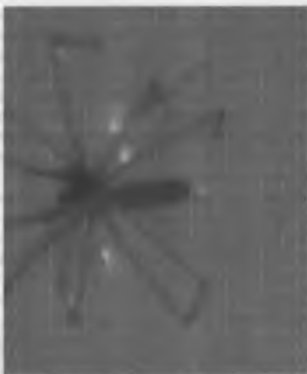
FIGURE 1.3 Insect strides on the surface of water.
