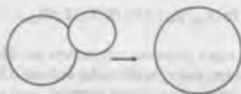
FIGURE 2.6 Coalescence of two bubbles with different radii.
