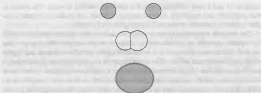
FIGURE 9.5 Two oil drops (top); flocculation step (middle); coalescence (bottom).
