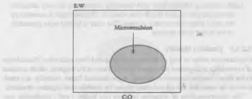
FIGURE 9.4 Four-component system: Oil (O)–Water (W)–Emulsifier (E)–Cosurfactant (S) (ratio of O:S versus S:W).
