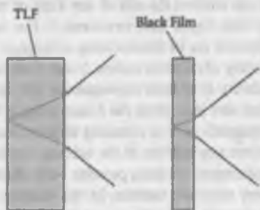
FIGURE 8.2 TLF and reflection of light.
