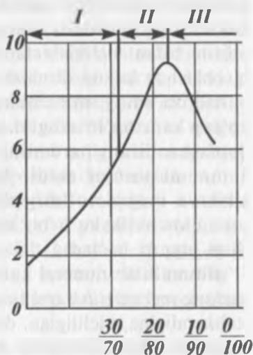
9.5-rasm. Mineral kukunining asfalt-beton mustahkamligiga ta'siri.
