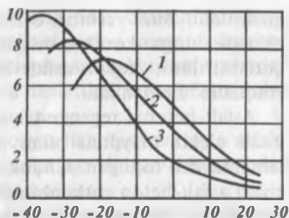
9.13-rasm. Asfalt-betonning egilishga bo'lgan mustahkamligiga haroratning ta'siri: 1 — YNB 60/90; 2 — YNB 130/200; 3 — YNB 200/300.
