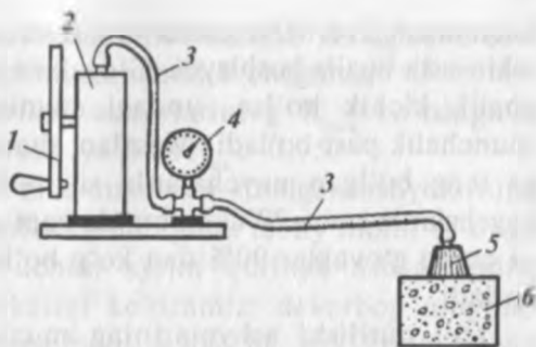
2.2-rasm. Betonning suv o'tkazuvchanligini tezkor usulda aniqlash.
