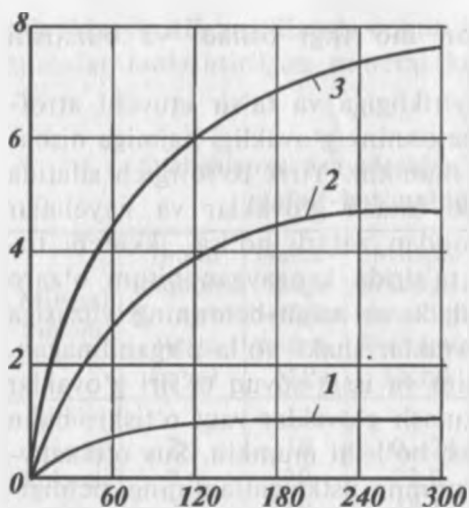
9.11-rasm. Asfalt-betonning suv shimuvchanligi: 1 — bitum mineral kukuni bo'tqasi; 2 — asfalt qorishma (bitum+mineral kukuni+qum); 3 — asfalt-beton
