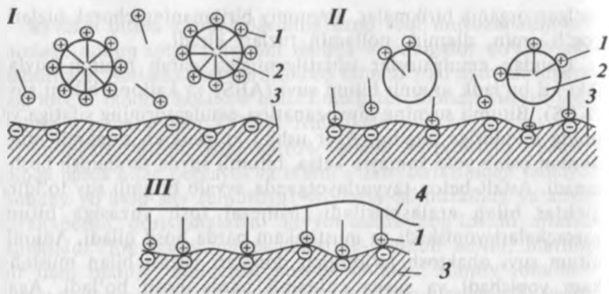
8.7-rasm. Kationli bitum suvida bitum pardasining hosil bo'lishi va tosh yuzasiga yopishishi: I—III—bitum zarrachalarining saralanishi. 1—emulgator; 2—bitum zarracha; 3—toshning yuzasi; 4—bitum pardasi.
