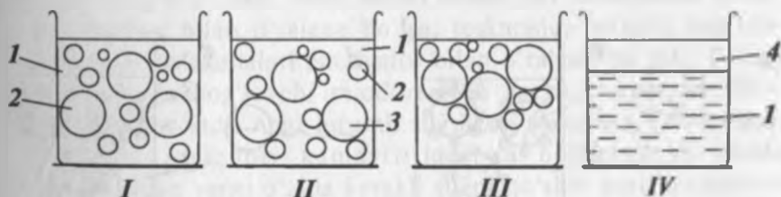
8.5-rasm. Emulgator qo'shilmagan suvdagi bitum zarrachalarining holati:
