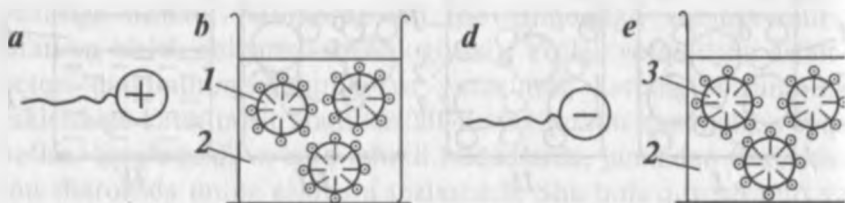
8.6-rasm. Emulgator qo'shilgan bitum suvi:
