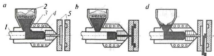
11.5-rasm. Bosim ostida quyish mashinasining ishlash sxemasi:
