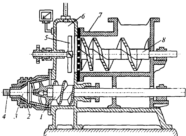
3.2-rasm. Tasmali vakuumli press:
