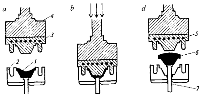
11.4-rasm. Press-qoliplash (shtamplash) sxemasi:
