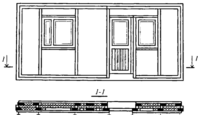
9.11-rasm. Devorbop asbosement panel.
