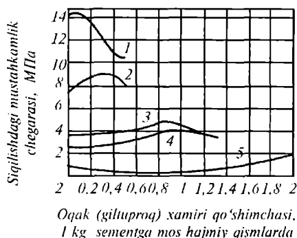
8.2-rasm. Kukun qo'shimchalarning (ohak, giltuproq) qorishma mustahkamligiga ta'sirini ifodalovchi bog'lanish. Sement: qumi (hajm bo'yicha): 1-1:3; 2-1:4; 3-1:5; 5-1:9.
