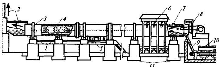
5.3-rasm. Aylanma xumdon:
