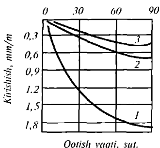
6.10-rasm. Kirishish chizmasi:
