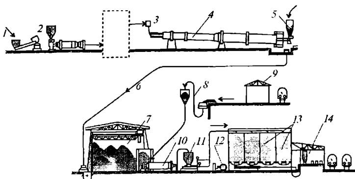
5.4-rasm. Portlandsement ishlab chiqarish sxemasi:
