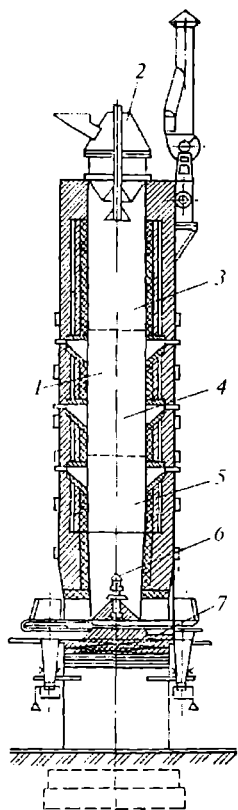
5. 1-rasm. Shaxtali xumdon:
