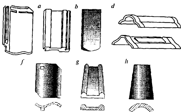
3.5-rasm. Keramik cherepitsaning turlari:
