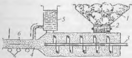
7-rasm. Yotiq lentali pressda g'isht quyish: 1–yuklaydigan voronka; 2–valiklar; 3–shnek; 4–press mundshutgi; 5–namlagich; 6–lentasimon sigma massa; 7–tayanuvchi rolıklar.
