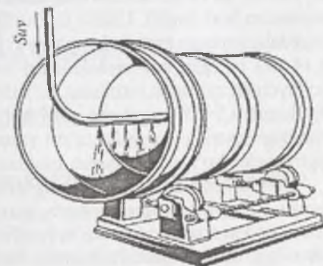
11-rasm. Toshsimon materiallarni yuvish barabani (shpatyuvgich).
