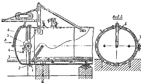
2.24-rasm. Bayonet yopqichli avtoklav:
