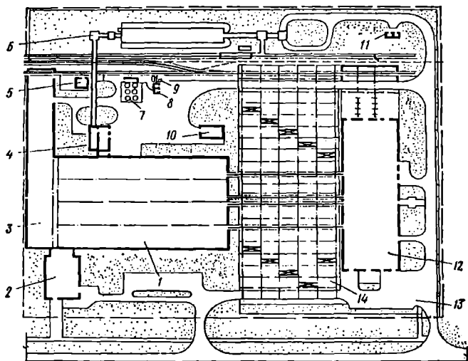
1.36-rasm. Yirik panelli uysozlik zavodining bosh loyihasi:
