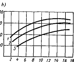
2.13-rasm. Portlandsement asosidagi beton mustahkamligining oshib borishi:
