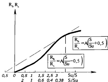
2.5-rasm. Su/S nisbatiga beton mustahkamligining bog'liqligi.
