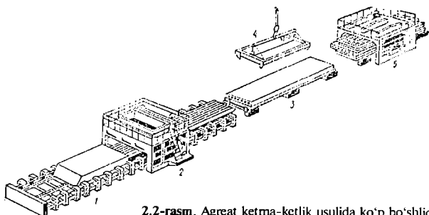
2.2-rasm. Agreat ketma-ketlik usulida ko'p bo'shliqli panellar tayyorlash uchun moslama: 1 — qoliplash mashinasi; 2 — beton yotqizuvchi; 3 — pod-don; 4 — avtomat tutqich; 5 — silkitish shiti va bortli o'zi yurar portal.
