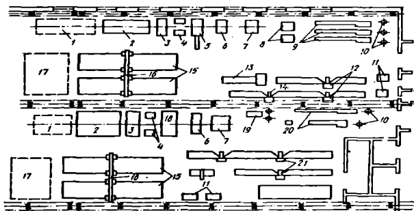
1.16-rasm. Uy-joy qurish kombinatining armatura sexi rejasi:
