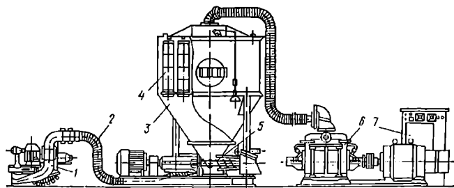
1.16-rasm. Sementni pnevmatik usulda tushirish chizmasi:
