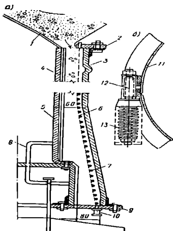
1.67-rasm. Trubani vibrogidroresslash usuli bilan qoliplash:
