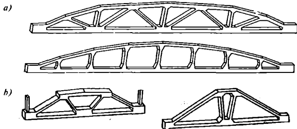
1.9-rasm. Stropil (a) va stropilosti (b) fermalar.
