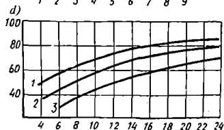
2.13-rasm. Portlandsement asosidagi beton mustahkamligining oshib borishi:
