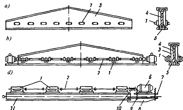
1.60-rasm. Yakka tartibdagi vibroqoliplar:
