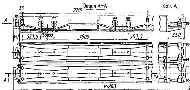
2.3-rasm. Ko'chma kuchlanish qolipi.
