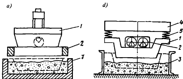
1.64-rasm. Beton qorishmasini vibroshtamplash jarayoni chizmasi:
