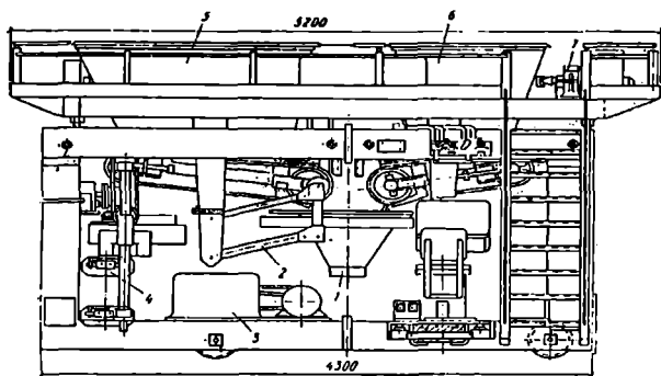
1.53-rasm. SMJ-166A nusumli beton yotqizgichning chizmasi:
