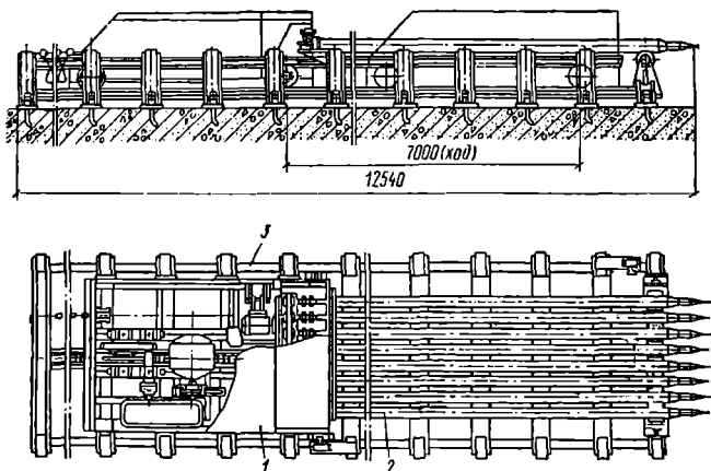
1.63-rasm. SMJ-227 rusumli qoliqlash mashinasining chizmasi:
