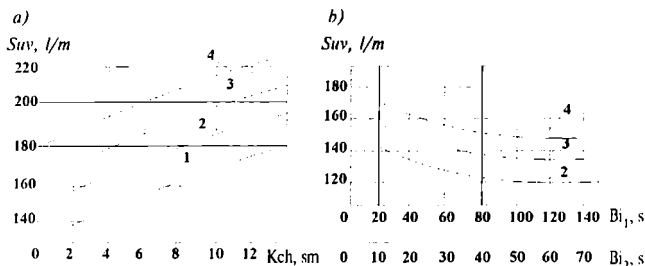
1.10-rasm. Portlandsement, o'rtacha yiriklikdagi qum (suv shimuvchanligi 7%) va yirik donador shag'aldan tayyorlangan plastik (a) hamda bikir (b) beton qorishmasining suv shimuvchanlik grafigi (Suv, l/m³).
