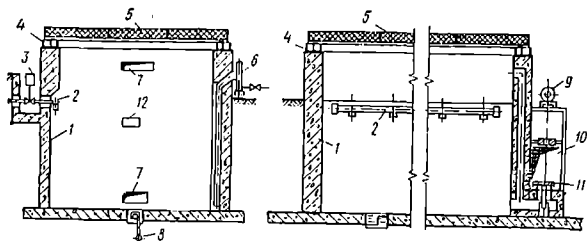
2.14-rasm. Handaq tipidagi bug'lash kamerasi:
