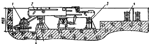
1.58-rasm. SMJ-280 rusumli vibromoslama chizmasi:
