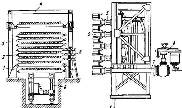
2.22-rasm. Termoformalami paketlovchi moslama:
