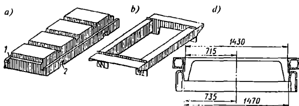
1.45-rasm. Orayopmalar (plita) uchun yig'ma qolip:
