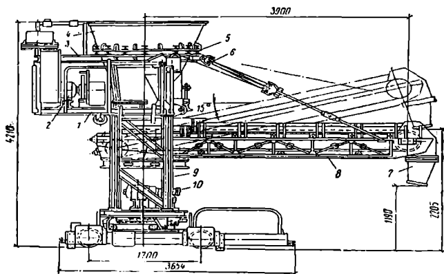
1.50-rasm. SMJ-71A beton taqsimlash mexanizmining tuzilishi:
