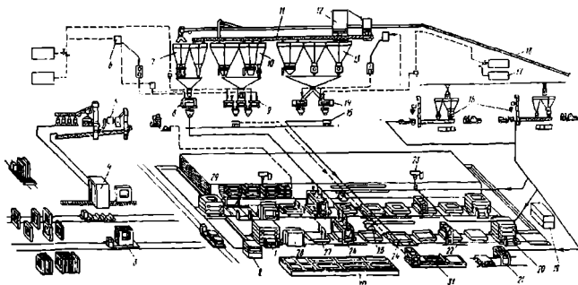
1.4-rasm. Tashqi devor panellarini tayyorlash.
