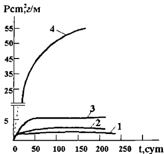
2.18-rasm. Namunalardagi po'lat zanglashining P_{cm} kinetikasi.
