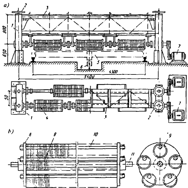
1.47-rasm. Tag asos (poddon)ni tozalash mashinasi:
