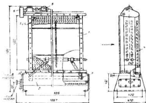
10.12-rasm. Kd 10006 o'zi tozalonovchi filtr.
