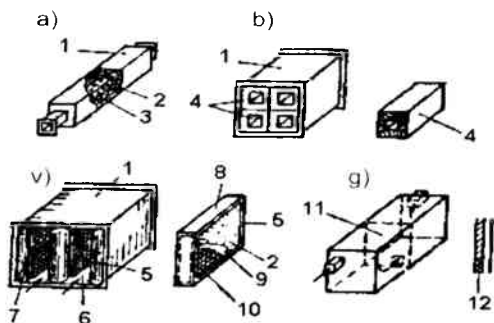
16.1-rasm. Shovqin so'ndirgichlarning chlzmalar.
