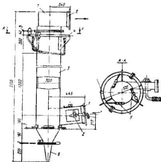
10.5-rasm. VTI Promstroyproyekt Skrubberi SS-3.
