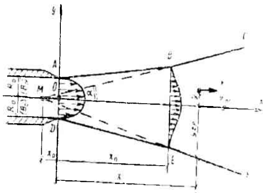
6.2-rasm. Erkin turbulent oqim.
