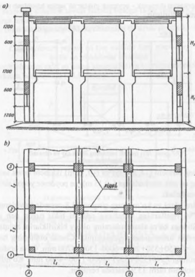
13.8-rasm. Binoning ko'ndalang qirgimi (a) va tarhi (b).
