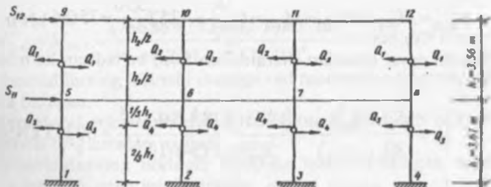
13.11-rasm. Ramaning hisoblash tashari.
