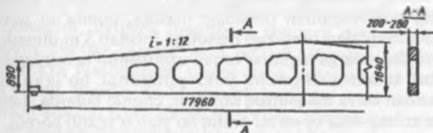
11.4-rasm. Ikki nishabli, oldindan zo'riqtirilgan, panjarali to'sin.
