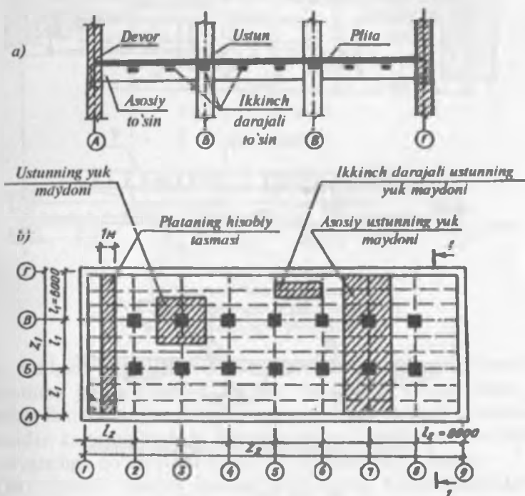
4.13-rasm. Bino tarhi:
