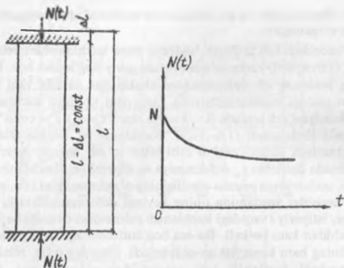
1.6-rasm. Betonda kuchlanishlarning kamayishi (relaksasiyalanishi).
