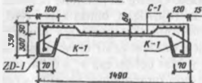
2-2 qirgim
