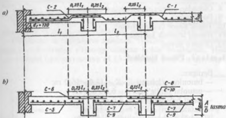
4.15-rasm. Plitani armaturalash:
