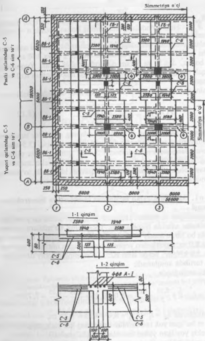
5.4-rasm. Ikkinchi darajali to'sinning tayanch qismini armaturalash.
