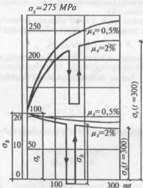
1.15-rasm. Beton tob tashlashidan temirbetonda kuchlanishlarning o'zgarishi.
