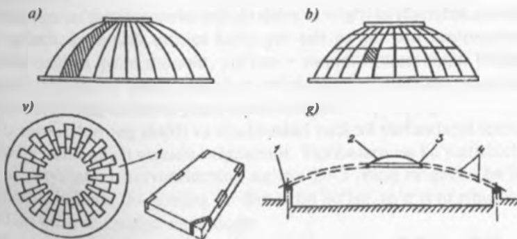
11.17-rasm. Yig'ma gumbazlar:
