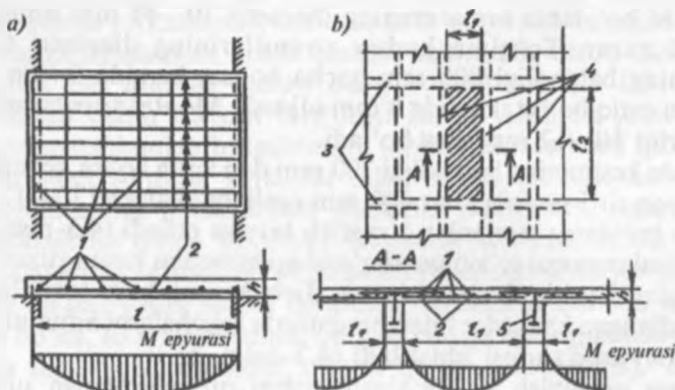
4.4-rasm. To'sinsimon yaxlit plitalarni armaturalash:
