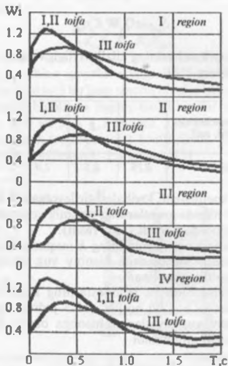
13.5-rasm. Spektral koeffitsienti W_1 grafigi.
