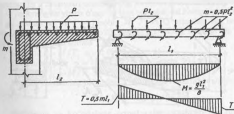
6.12-rasm. To'sinning buralib egilishini hisoblashga doir.
