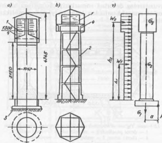
12.5-rasm. Suv bosimi minoralari (a, b) va ag'darilishga hisoblash tarhi (v): a — temirbeton silindrik tayanch; b — rama tayanch.
