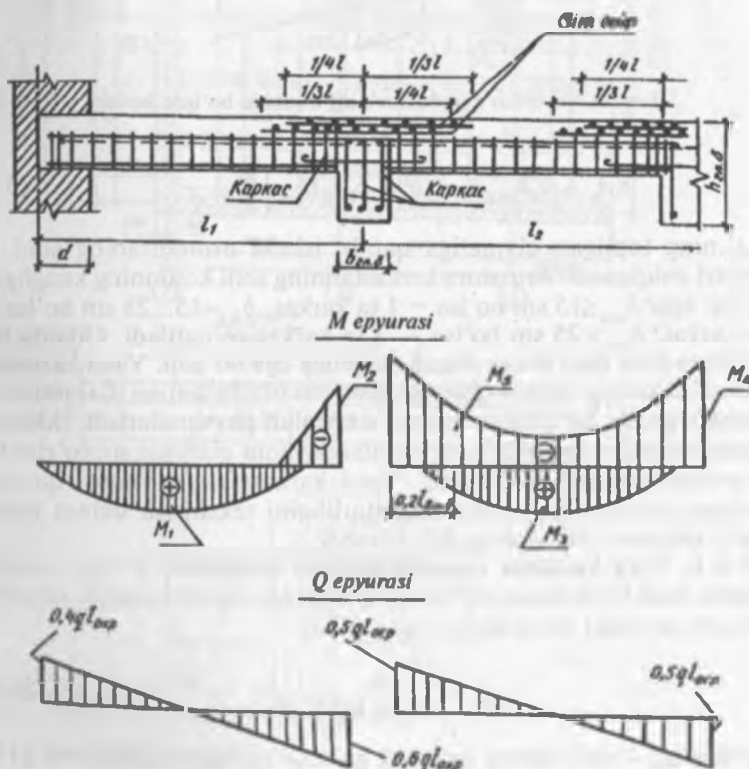
5.2-rasm. Ikkinchi darajali to'sinni armaturalash.
