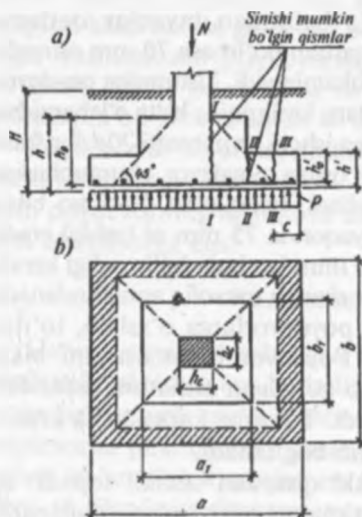
9.2-rasm. Alohida poydevor (poyustun)ni hisoblashga doir:
