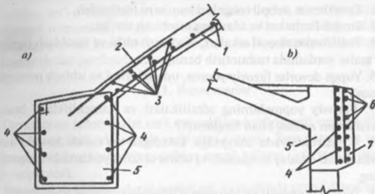
11.16-rasm. Quyma gumbazni armaturalash:
