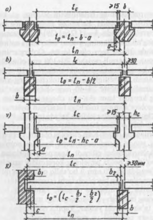
6.2-rasm. Panellarning rigelga tayanish usullari.
