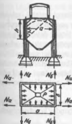
12.6-rasm. Bunker hisobiga doir.
