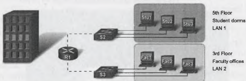
3.12-rasm. VLAN.
