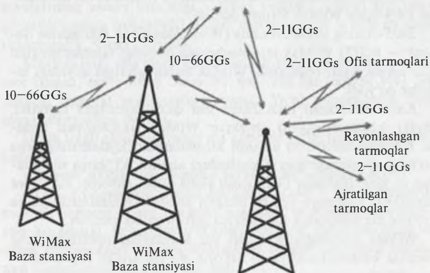
3.8-rasm. WiMAX antennalari bog'lanishi.
