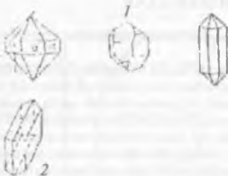
2.2-rasm. Ayrim minerallar kristallari shakli.
