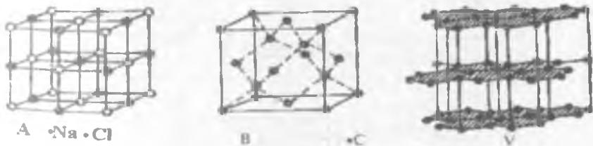
2.1-rasm. Ayrim minerallarning kristall turlari.
