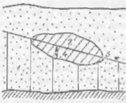
7.5-rasm. Mahalliy bosimning vujudga
