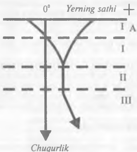
1.2-rasm. Yerning ichida haroratning taqsimlanish chizmasi
