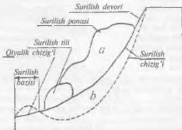
6-1-rasm. Surilish bazisining yotish sxemasi:
