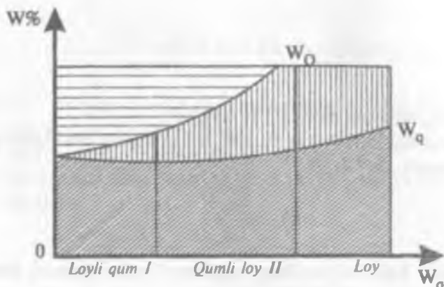
8.1-rasm. Loyli grunt holatini ifodalovchi chizma
