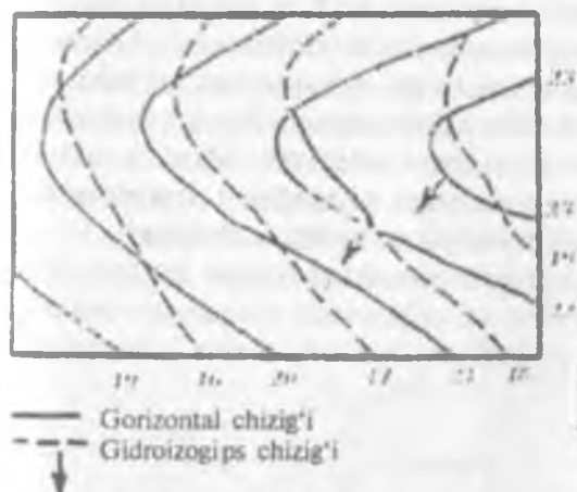
7.6-rasm. Gidroizogips xartasi: 1-gorizontal chiziq; 2-gidroizogips chizig'i;
