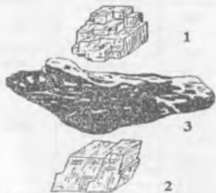
2.4-rasm. Minerallarning birikish turi.
