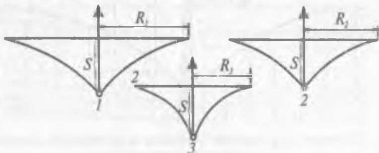
7.15-rasm. Depression voronkalar;
