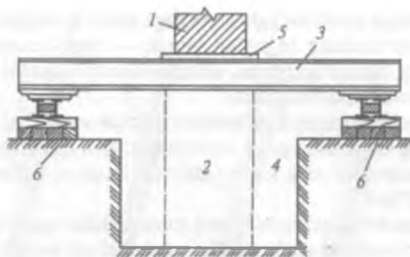
27- rasm. Ko'taruvchi to'sin(ranbalka) yordamida poydevorni osish:
