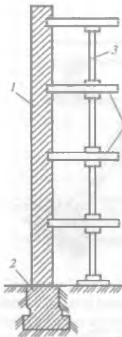
29- rasm. Vaqtinchalik tayanchlar yordamida tasmasimon poydevor yukini yengillashtirish sxemasi: 1—devor; 2—eski poydevor; 3—ustun; 4—orayopma.
