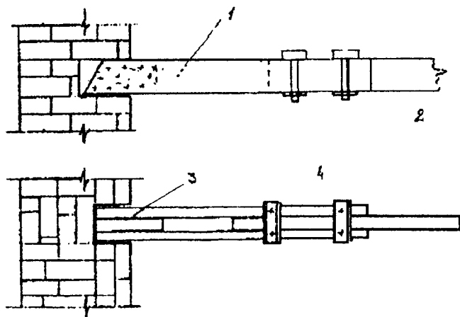
9.9-rasm. Orayopma balkasining tayanch qismini kuchaytirish.
