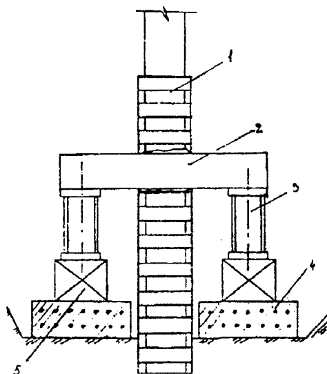
9.2-rasm. Tasmaimon poydevorni yordamchi tayanch bilan kuchaytirish.
