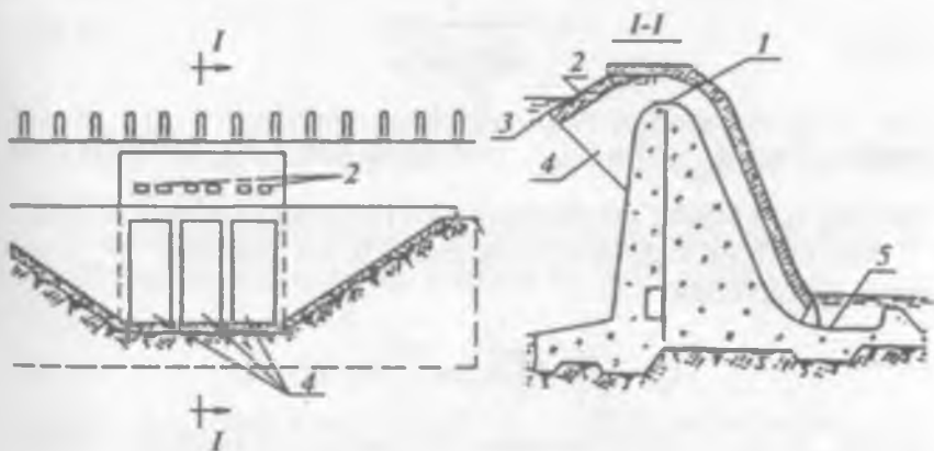
2.8- rasm. Sifonli suv tashlagich:
