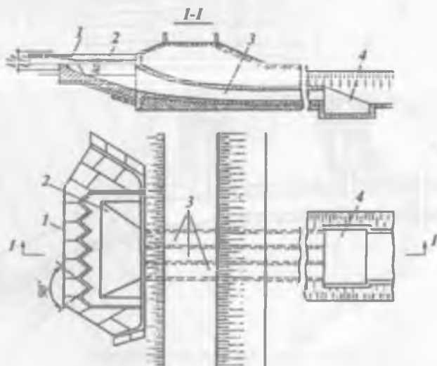
2.11- rasm. Cho'michsimon suv tashlagich:
