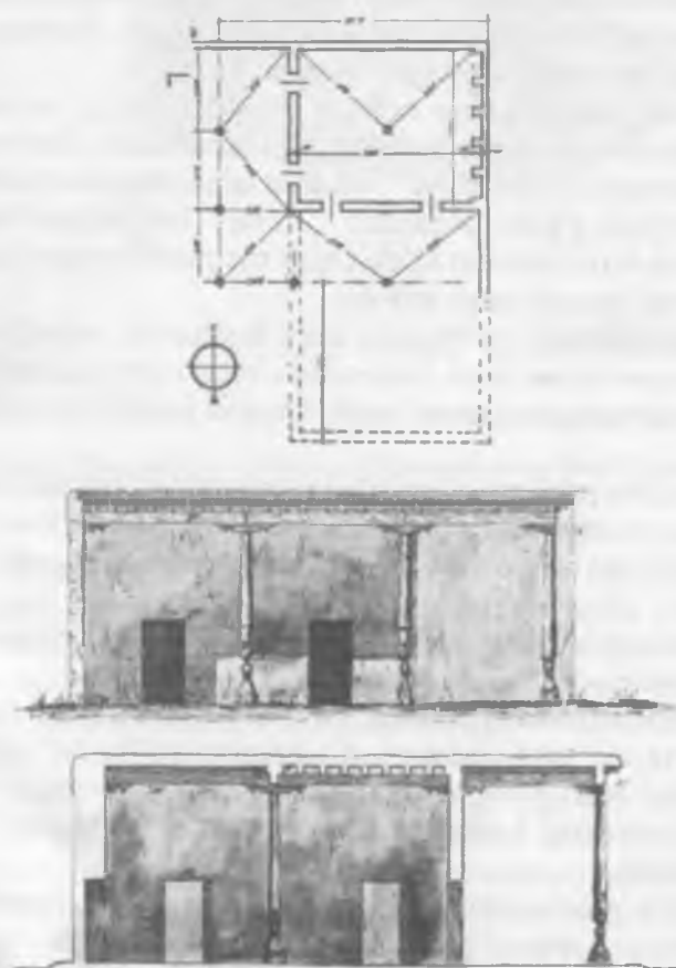
6.4.1-rasm. Guzar masjidi, tarh, tarz, qirqim chizmalari.
