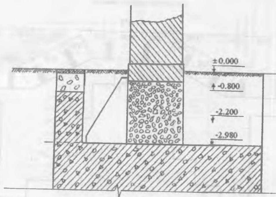
4-rasm. Poydevor qirgimi.
