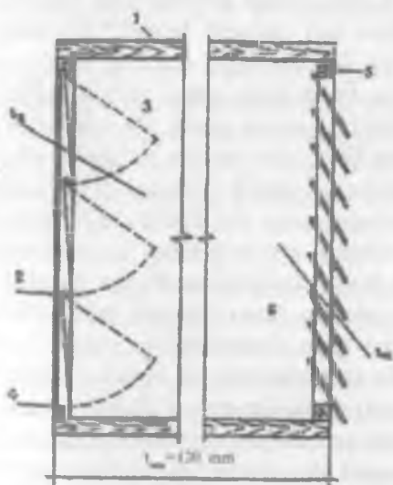
4.4.4-rasm. Ventilatsiyali klapan qurilmasi: 1-qobiq; 2-o'q; 3-sterjen; 4-klapan (jez, b-0.2 mm); 5-oldingi rom; 6-orqa rom; 6-darpardalar.
