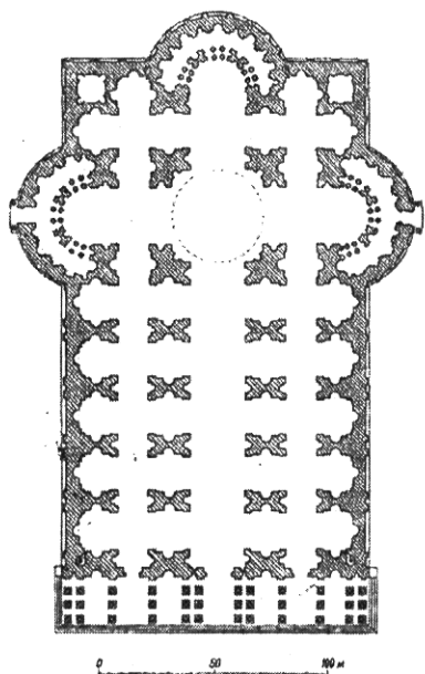
Римдаги авлиyo Pyotr sobori. Planlar: a) Bramante-1505 y. b) Rafael Santi – 1514 y. v) A.Sangallo-1536 y. g) Mikelandjelo-1547 y.
