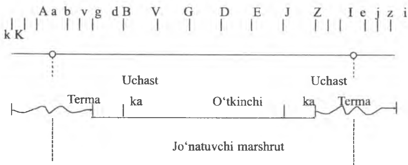
4.5 – rasm. Jo'natuvchi marshrutning harakatlanish sxemasi
