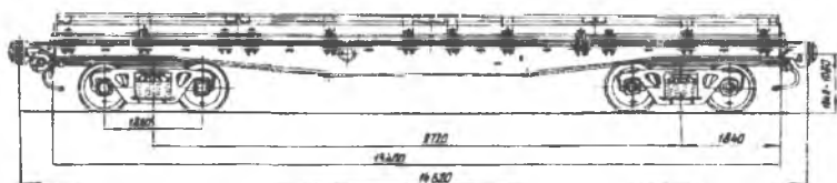
5.8.2-rasm. Universal to'rt o'qli platforma
