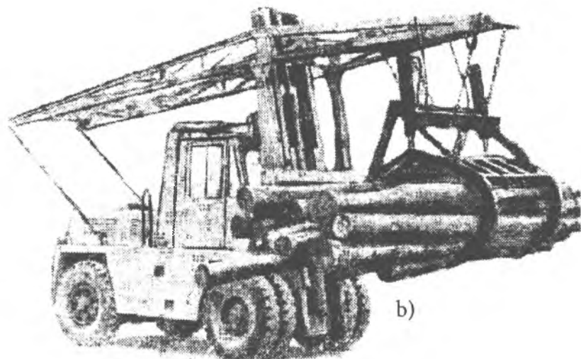
5.15-rasm. Avtoyuklagichlar; a) 4008, b) 4028
