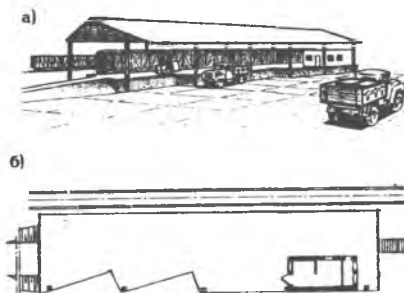
6.6 - rasm. Tishsimon rampali yopiq yuk platformasi: a – umumiy ko‘rinishi; b – tarhi
