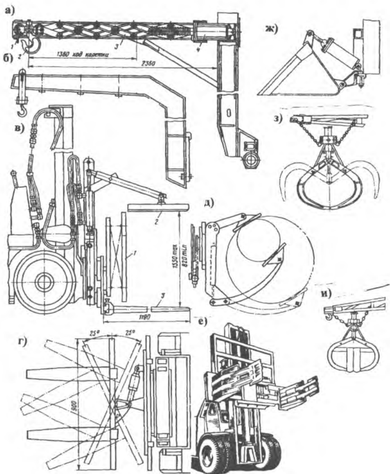
5.16-rasm. Donali yuklarni ilib olish va sochiluvchan-to'kiluvchan yuklarni botirib olish moslamalari.
