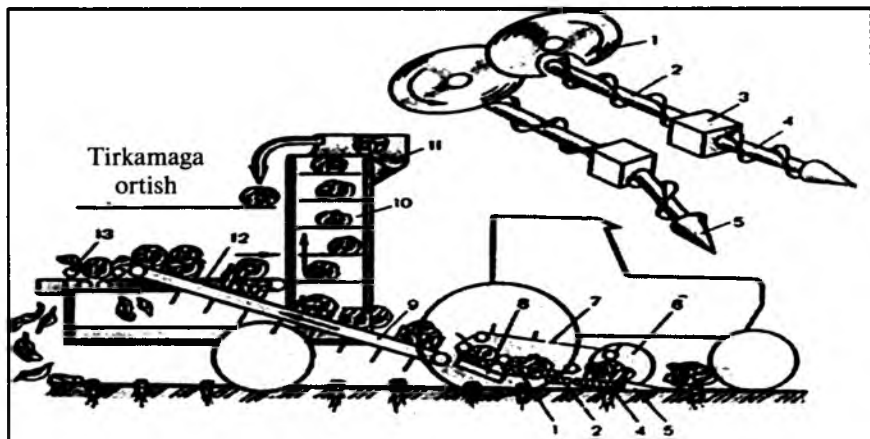
2.46-rasm. MSK-1 karam yig'ish mashinasining tuzilishi va ish jarayoni:
