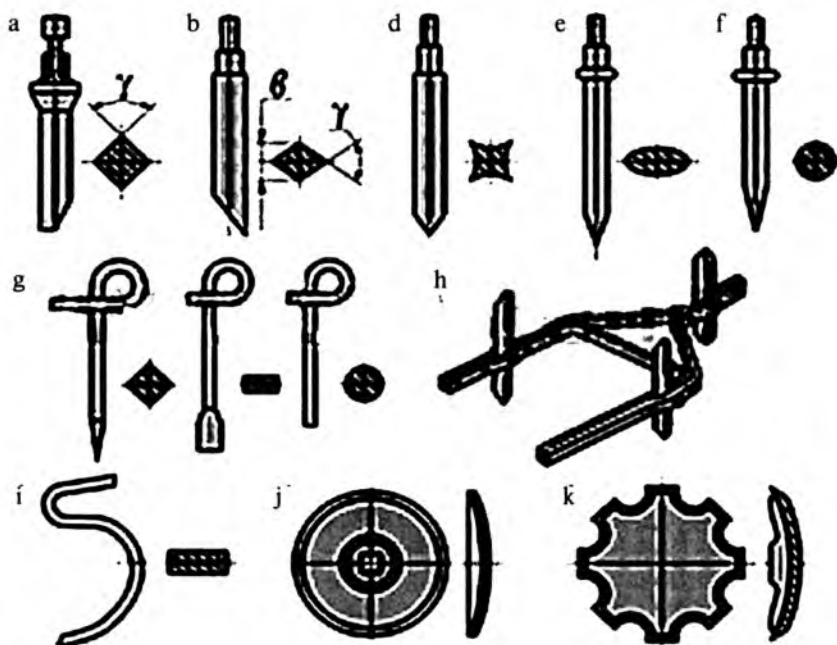
2.9-rasm. Borona tishlarining turlari:
