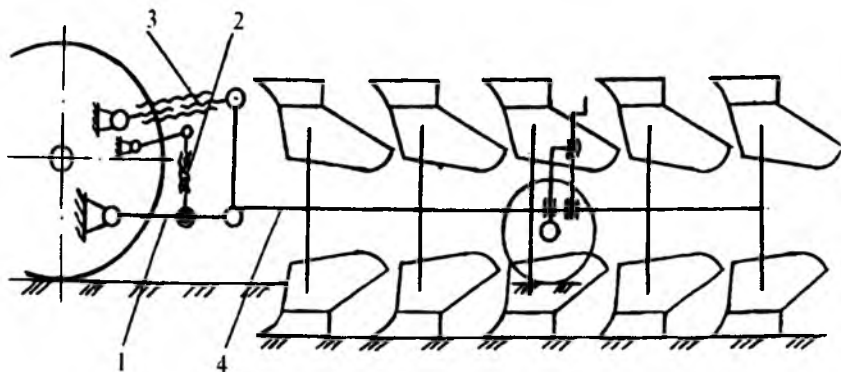
2.5-rasm. Osmo plug ramasini dala yuzasiga nisbatan paralleligini rostlash: 1 – traktor o'rnatish qurilmasining pastki tortqisi; 2 – pastki tortqining kashagi; 3 – markaziy tortqi; 4 – plug.
