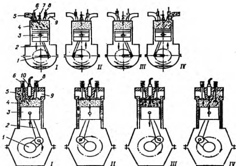
1.6-rasm. To'rt taktli karbyuratorli (a) va dizel dvigatellarning (b) ishlash sxemasi: 1 – tirsakli val; 2 – shatun; 3 – porshen; 4 – silindr; 5 – kiritish truboprovodi; 6 – kritish klapani; 7 – o't oldirish svechasi; 8 – chiqarish klapani; 9 – chiqarish truboprovodi; 10 – forsunka; I – kiritish; II – siqish; III – kengayish; IV – chiqarish.
