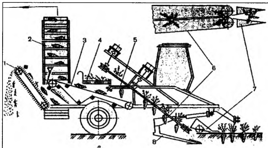
2.47-rasm. Ye-825 sabzi yig'ish mashinasining tuzilishi va ish jarayoni: 1 — chiqindi tozalagich; 2, 4 — transporterlar; 3 — elagich; 4 — silkitgich; 5 — barg ajratish apparati; 6 — silkitgich; 7 — barg ko'targich; 8 — lemex-kovlagich.
