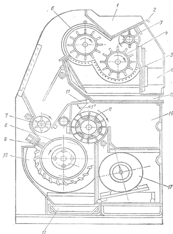
11-rasm. LKM rusumli asbob chizmasi
