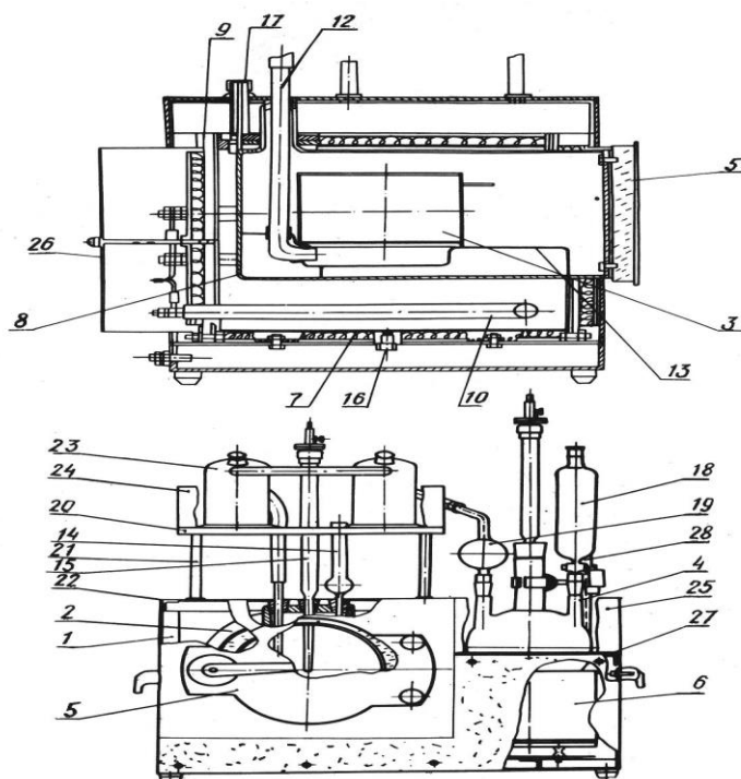
36-rasm. OSX - 1 chigit tuksizlantirgichning chizmasi
