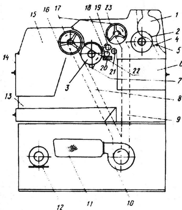
12 - rasm. PPV jin - tola tozalagichning chizmasi
