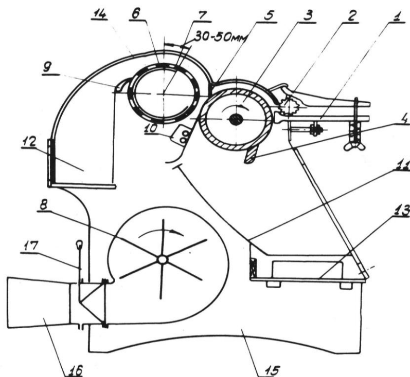
15-rasm AX-2 paxta analizatorining chizmasi
