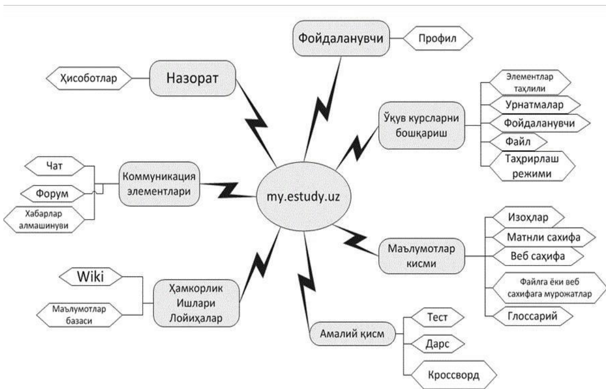
5.6.5-rasm.my.estudy.uz LMS tizimining strukturasi
