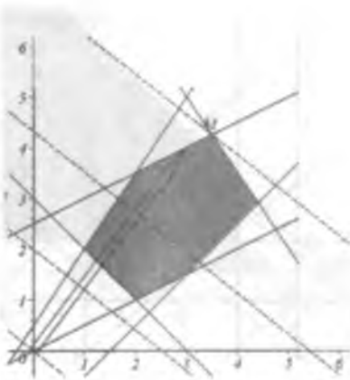
2.8-rasm. Yechim yagona (M nuqta)
