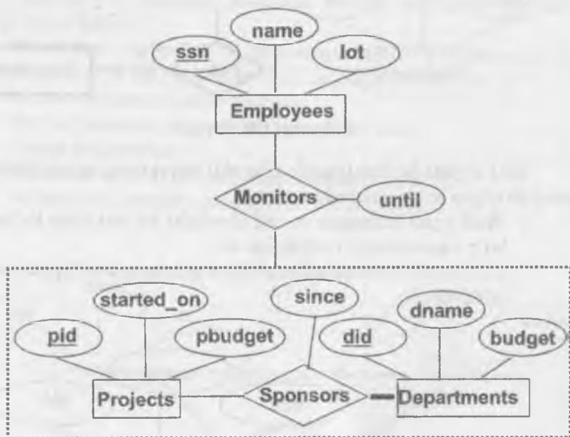
2.9-rasm ISA modeli
