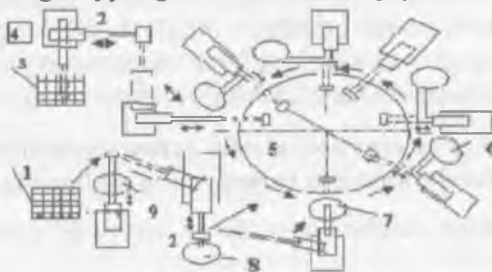
7.2 - rasm. Moslashuvchan robotli RTK:
