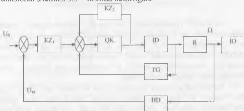
3.5 - rasm. Taqlidli elektrik yuritmaning funksional sxemasi:
