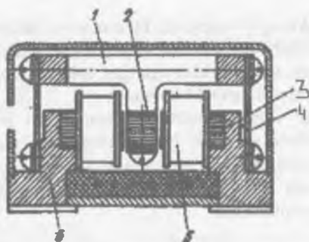
12.3 - rasm. Tezlanishni o'lchash uchun datchik
