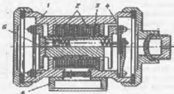
12.2 – rasm. Vibratsion siljishlar datchigi
