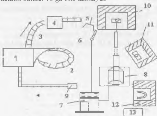
8.7-rasm. Issiq shtamplash RTKsi:
