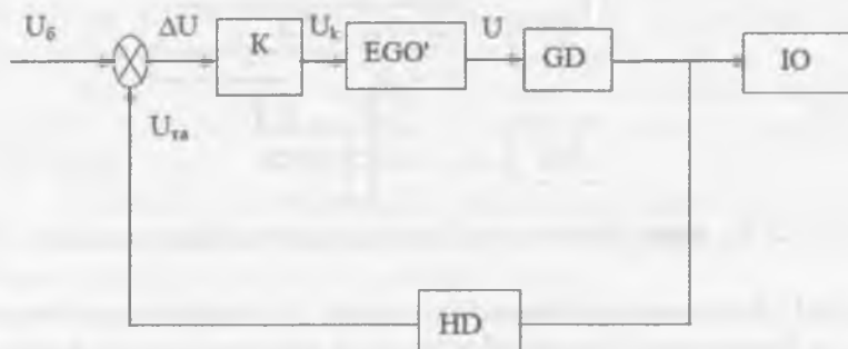
3.3 – rasm. Sanoat roboti elektrogidravlik yuritmasining funksional sxemasi:
