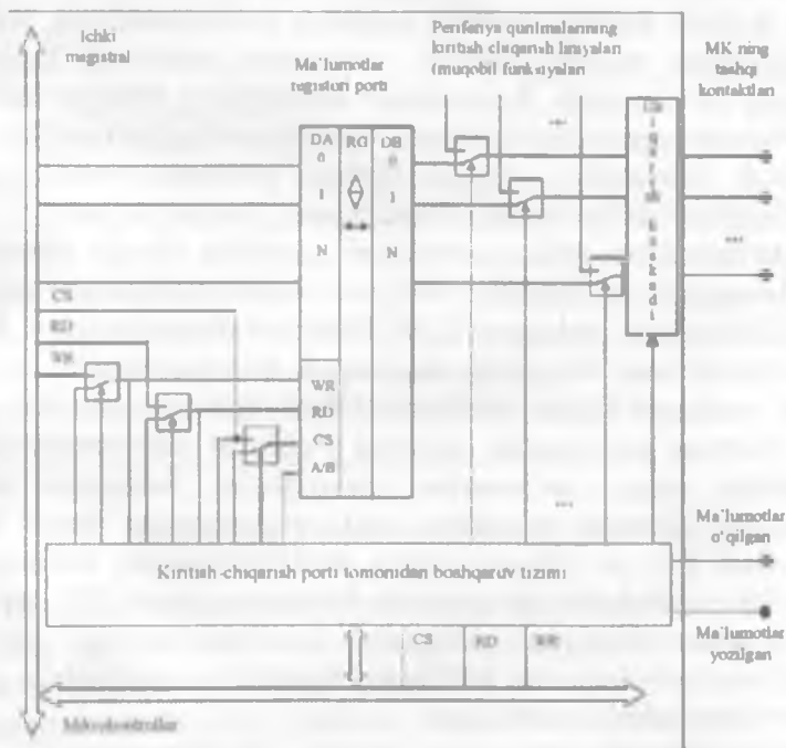
4.8-chizma. Kiritish chiqarishning parallel porti tuzilmasi
