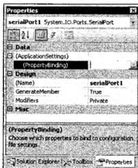
Рис. 10.6. Свойство (ApplicationSettings)
