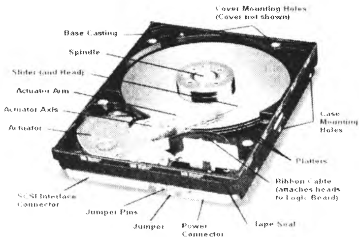
3.10-rasm. Mikrokompyuterdagi qattiq disk 6 .
