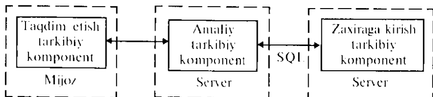
10.6-rasm. Qo'llanish (ilovalar) serverli modeli.
