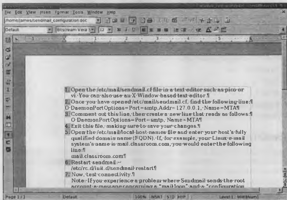
Рис. 11.20. Star Writer
