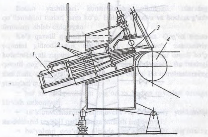
21-rasm. Uch kanalli Stratoflo qurilmasi:
