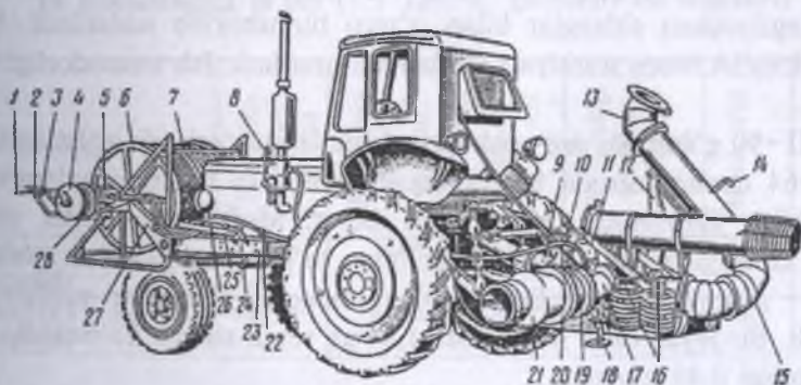
28-rasm. ППА–165У universal kó'chma sug'orish agregati:
