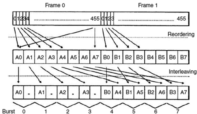
5.6-rasm. TCH/FS o'zgarish tartibi.
