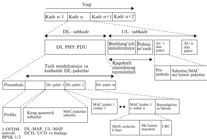
29.4-rasm. TDDli OFDM kadrning tuzilmasi.
