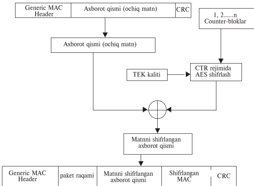
36.5-rasm. Xabarni axborot qismini shifrlash.
