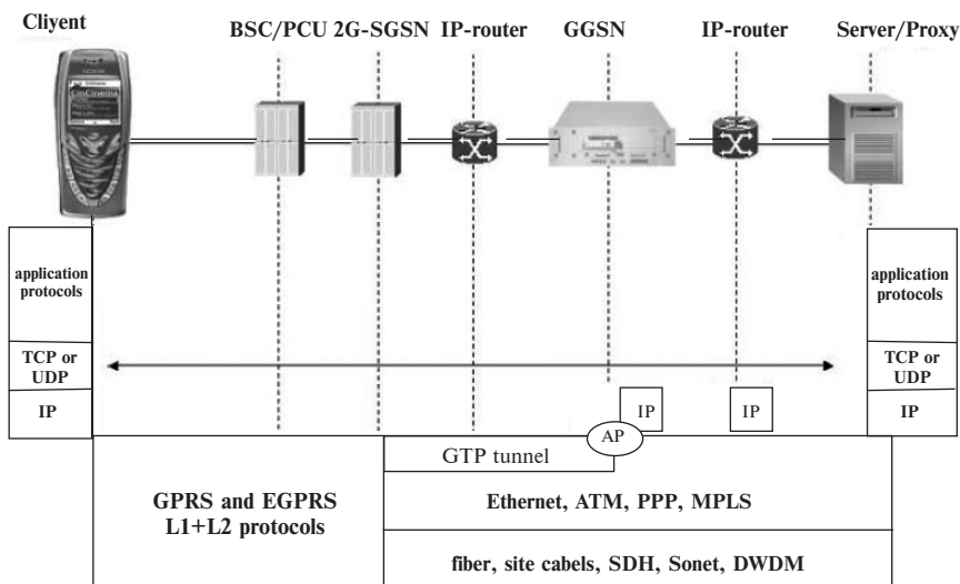
3.5-rasm. IP paketidan GPRS protokoliga o'tish.
