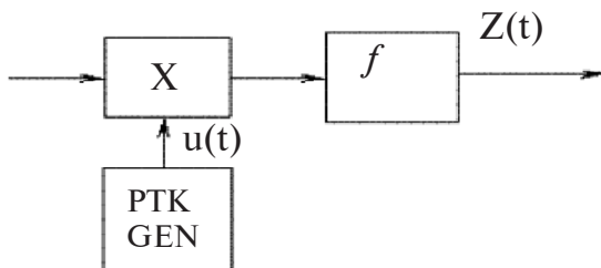
12.3-rasm. Keng polosali (shovqinsimon) signalning (SHPS) korrelyatsion qabul qilgichi.
