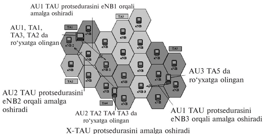
16.5-rasm. “Noaktiv LTE” holatida ko‘p sonli TAlar sxemasining ishlashi.
