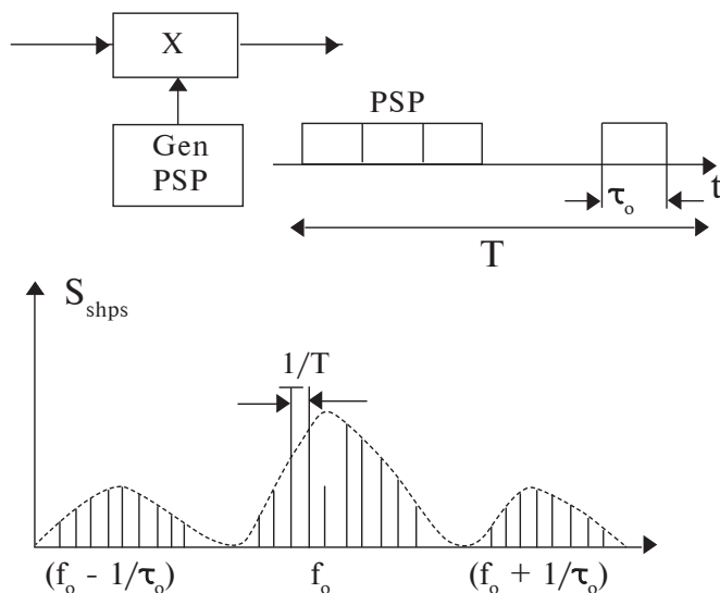
12.1-rasm. Chastota spektrini to‘g‘ridan to‘g‘ri kengaytirish usuli bilan keng polosali (shovqinsimon) signalni shakllash.
