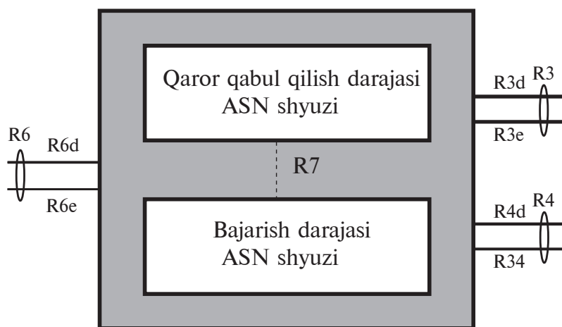
28.4-rasm. ASN shlyuzning tayanch nuqtalari.
