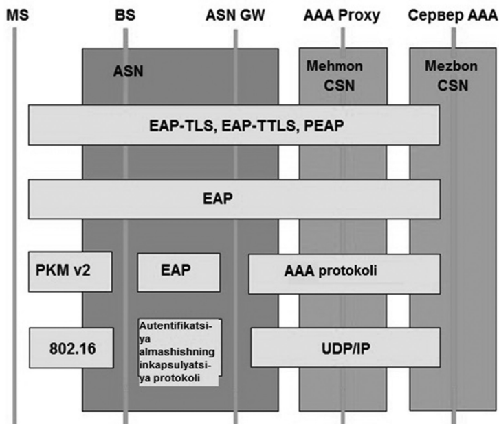
36.8-rasm. WiMAX tizimida AAA uchun protokollar steki.
