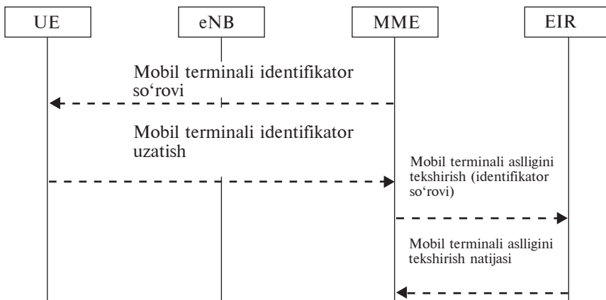
23.3-rasm. Abonent uskunasi (mobil terminal) aslligini tekshirish jarayoni.
