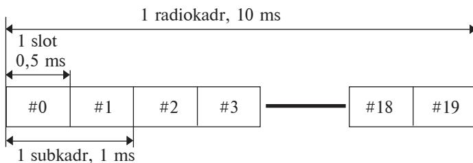
19.7-rasm. LTE radiokadrining FDD rejimi uchun tuzilishi.
