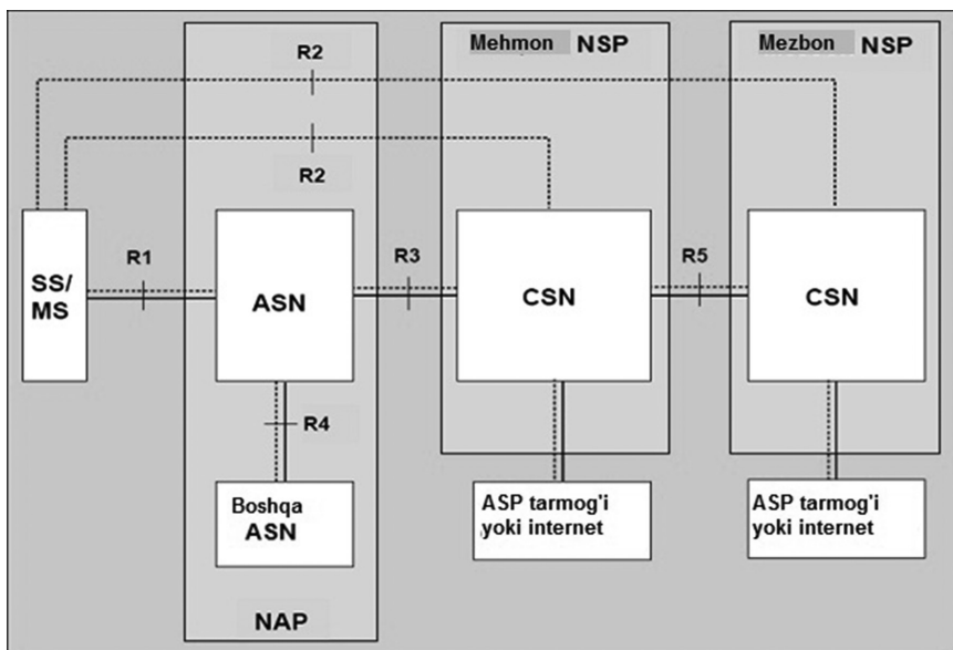
28.1-rasm. WiMAX tarmog‘ining tayanch modeli (NRM).
