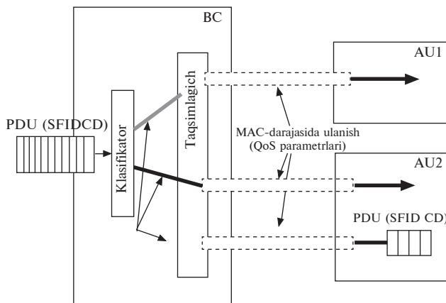
29.5-rasm. IEEE standartida QoSni qo‘llab-quvvatlash.
