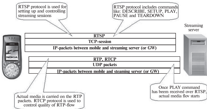
3.9-rasm. Audio/video ma'lumotlarini IP protokoli orqali yuborish.
