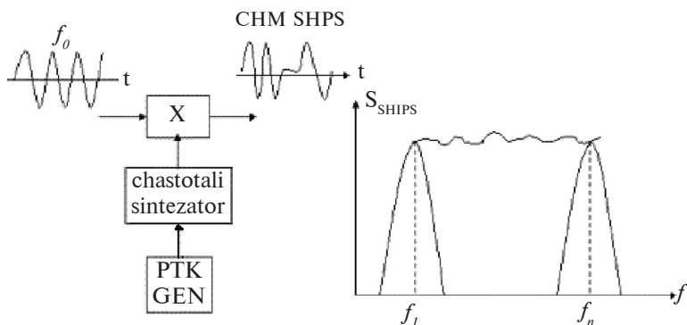
12.2-rasm. Chastotali sintezator.
