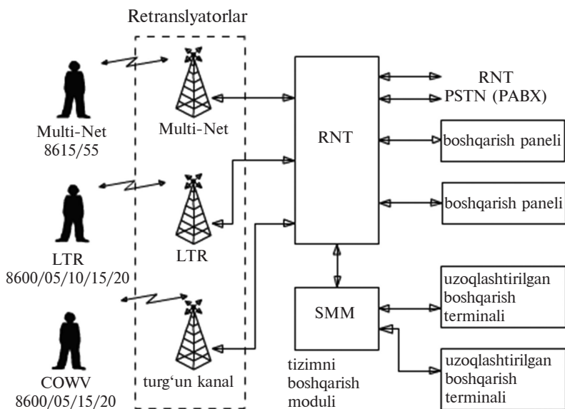
10.4-rasm. Kanallarning qaydlangan taqsimlanishli Multi-Net LTR tarmog'i.
