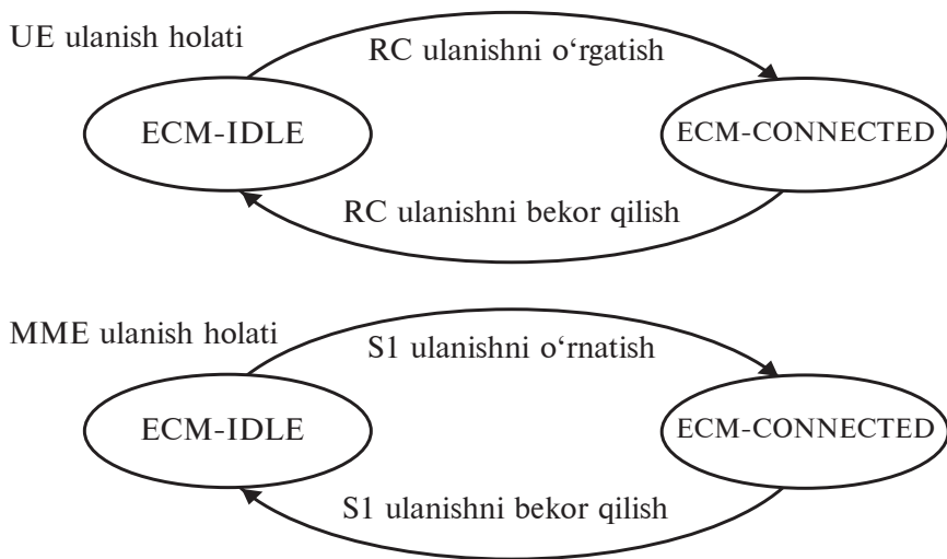
16.3-rasm. ESM darajasida AUning mobillik holatlari.
