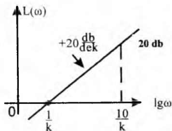
4.13-rasm. Differensiallovchi zveno uchun LChX.
