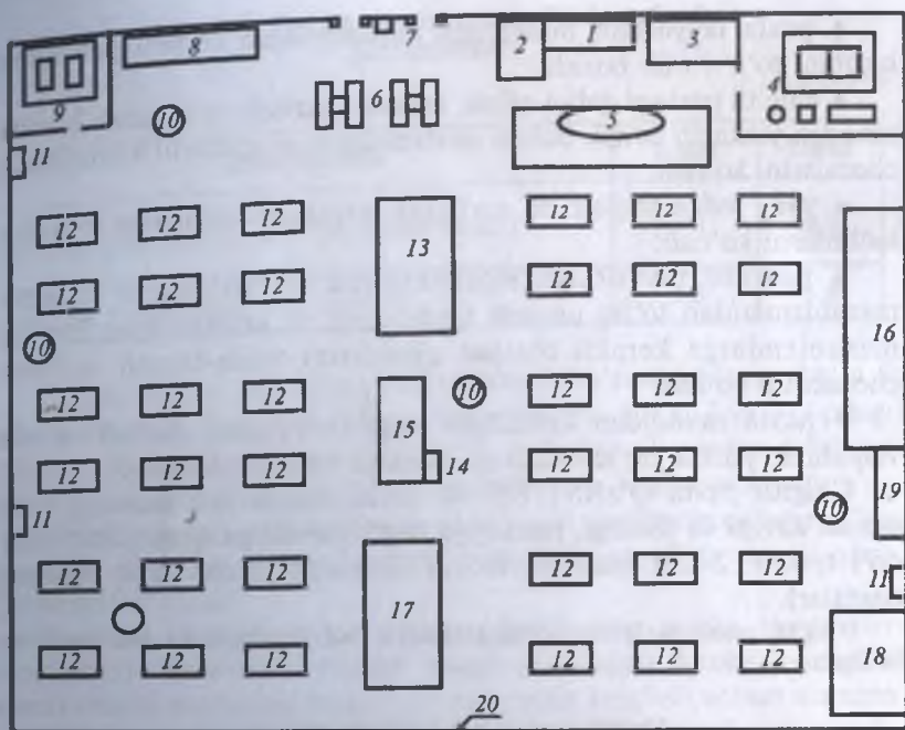
2-rasm. Namunaviy paxta tayyorlov maskanining bosh plani.
