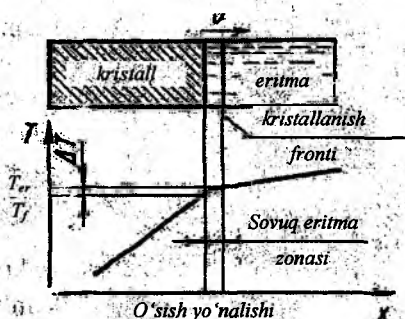
II.33-rasm. Suyuqmadan yo'nalgan kristallanish usulida kristall o'stirishda temperatura taqsimoti.
