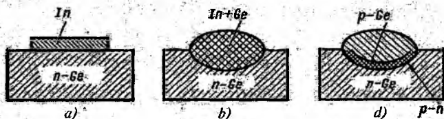
III.55-rasm. Qotishmali p - n o'tish tuzilmasining hosil bo'lishi
