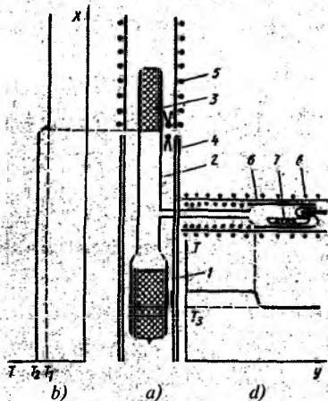
II.45-rasm. Monokristallarni bug' fazasidan (a) o'stirish va pechlar temperaturalari taqsimoti (b, d):
