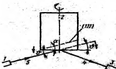
III.1-rasm. Quyma yo'nalishini rentgen usuli sxemasi:
