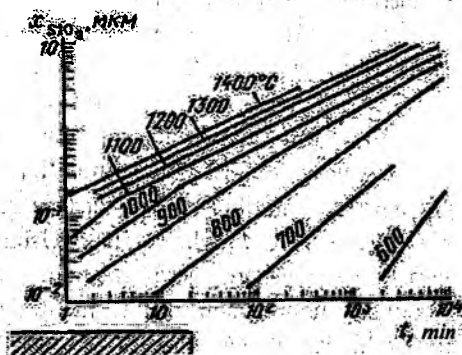
III.40-rasm. Suv bug'i muhitida turli temperaturalarda o'stirilgan \text{SiO}_2 parda qalinligining vaqtga bog'liqligi. 1- 600^{\circ}\text{C} ; 2- 700^{\circ}\text{C} ; 3- 800^{\circ}\text{C} ; 4- 900^{\circ}\text{C} ; 5- 1000^{\circ}\text{C} ; 6- 1100^{\circ}\text{C} ; 7- 1200^{\circ}\text{C} ; 8- 1300^{\circ}\text{C} ; 9- 1400^{\circ}\text{C} .
