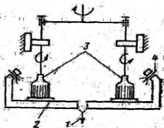
III.10-rasm. Gidromexanik yuvib tozalash jarayonining sxemasi:
