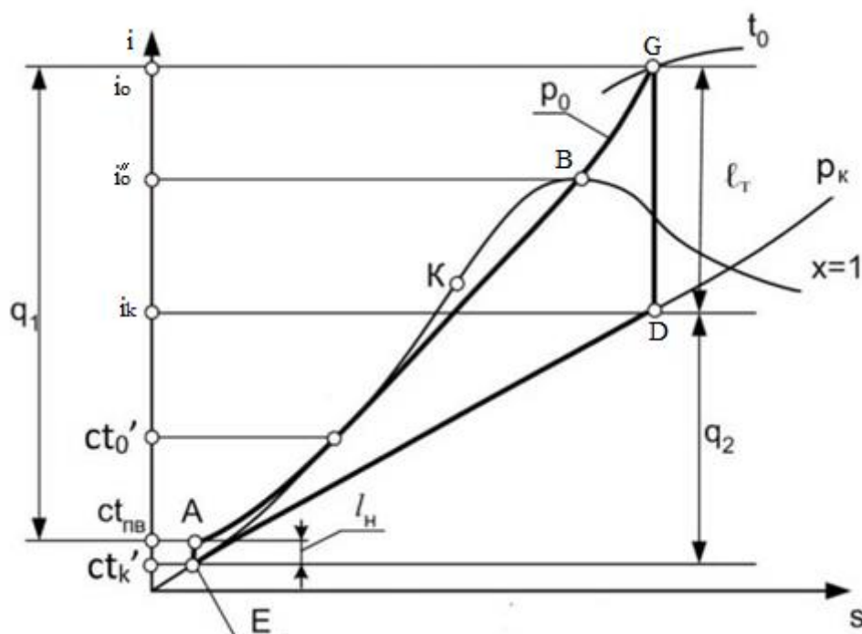
1.14-rasm. I,s - diagrammaga BKU sikli
