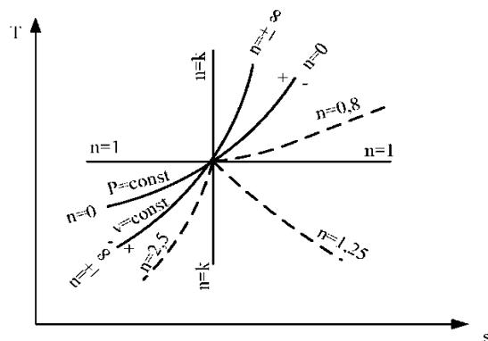
1.2-rasm. T, s - diagrammadagi ideal gazlar holati o'zgarishining politropoli jarayonlari
