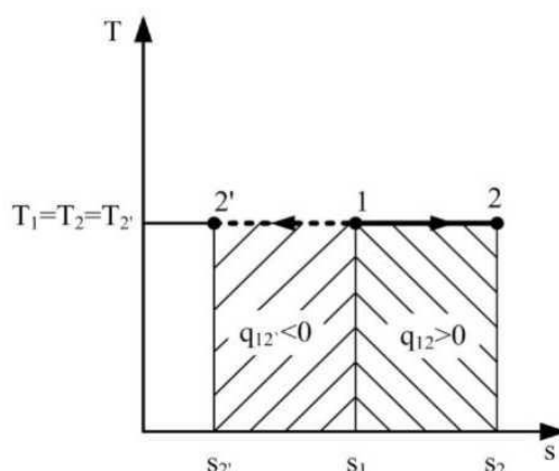
1.3-rasm. Ideal gaz kengayishi va siqilishining izotermik jarayoni
