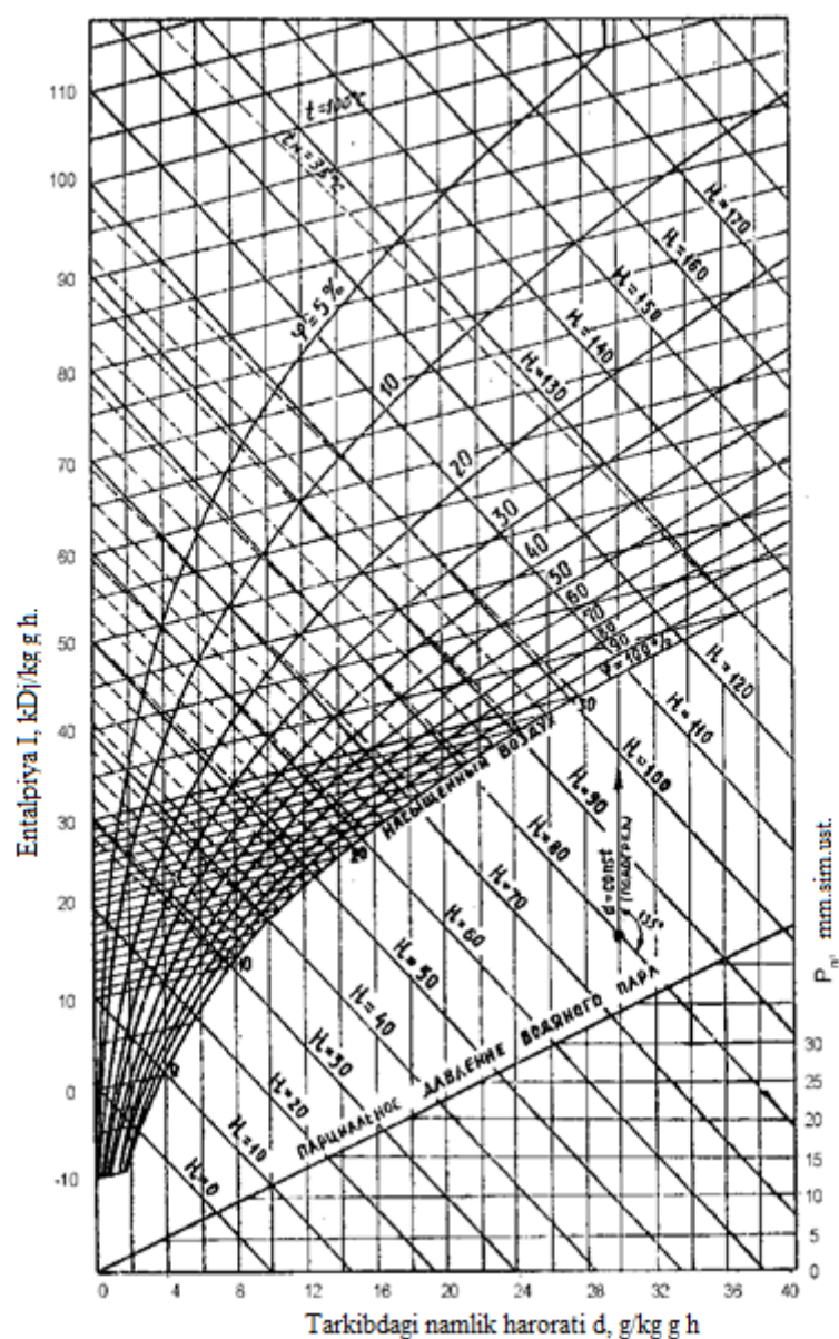
1.9-rasm. R = 745 mm. sim. ust. bo'lganida nam atmosfera havosining I,d - diagrammasi
