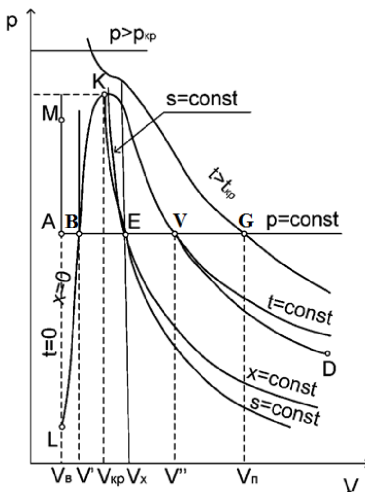
1.6-rasm. Suv bug`ining fazaviy ( p, v ) - diagrammasi
