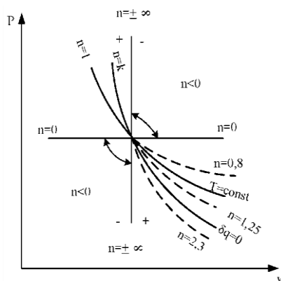
1.1-rasm. p, v - diagrammalarda ideal gazlar holati o'zgarishining politropoli jarayonlari
