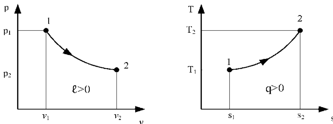
1.4-rasm. Ideal gazning p, v - va T, s - diagrammalardagi politrop kengayish jarayoni ( n=0,4 ).
