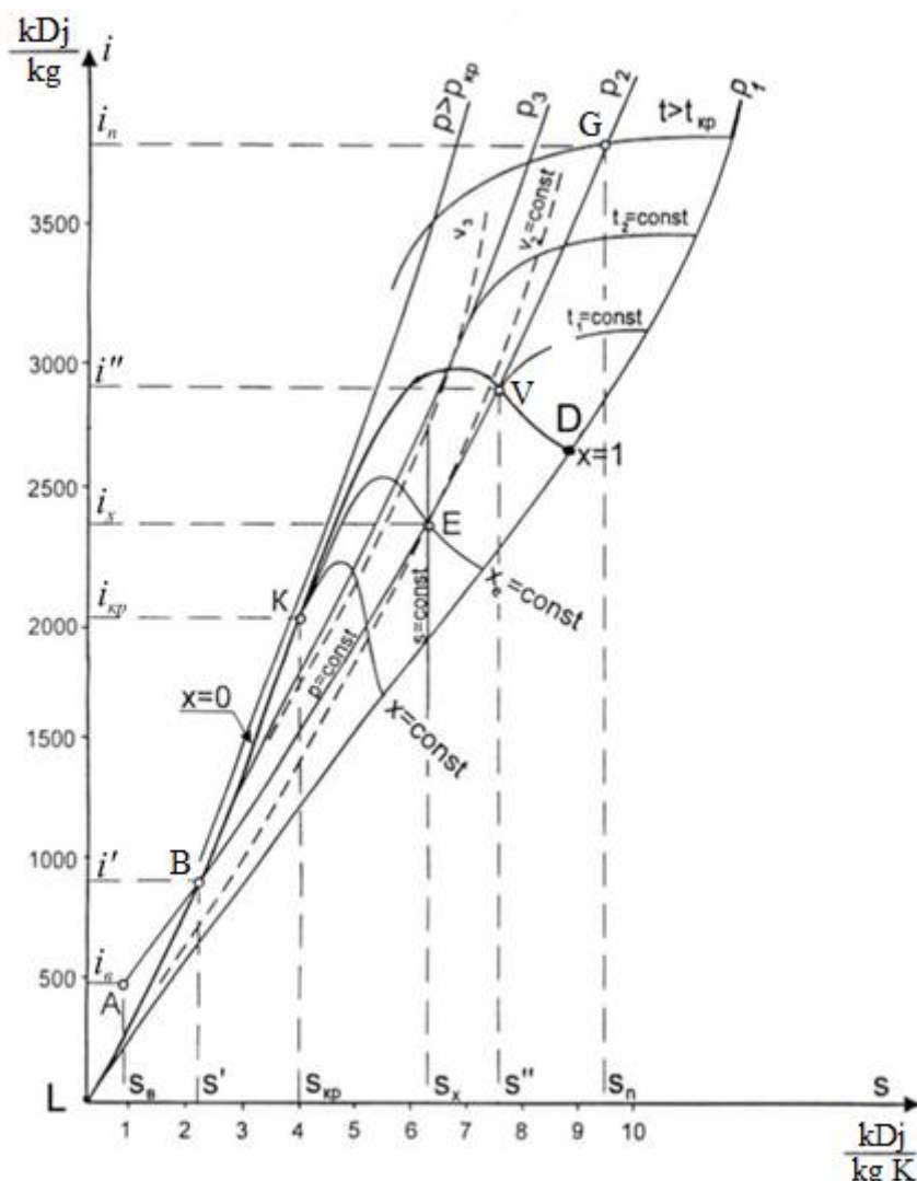
1.8-rasm. Suv bug'ining fazaviy (i, s) – diagrammasi
