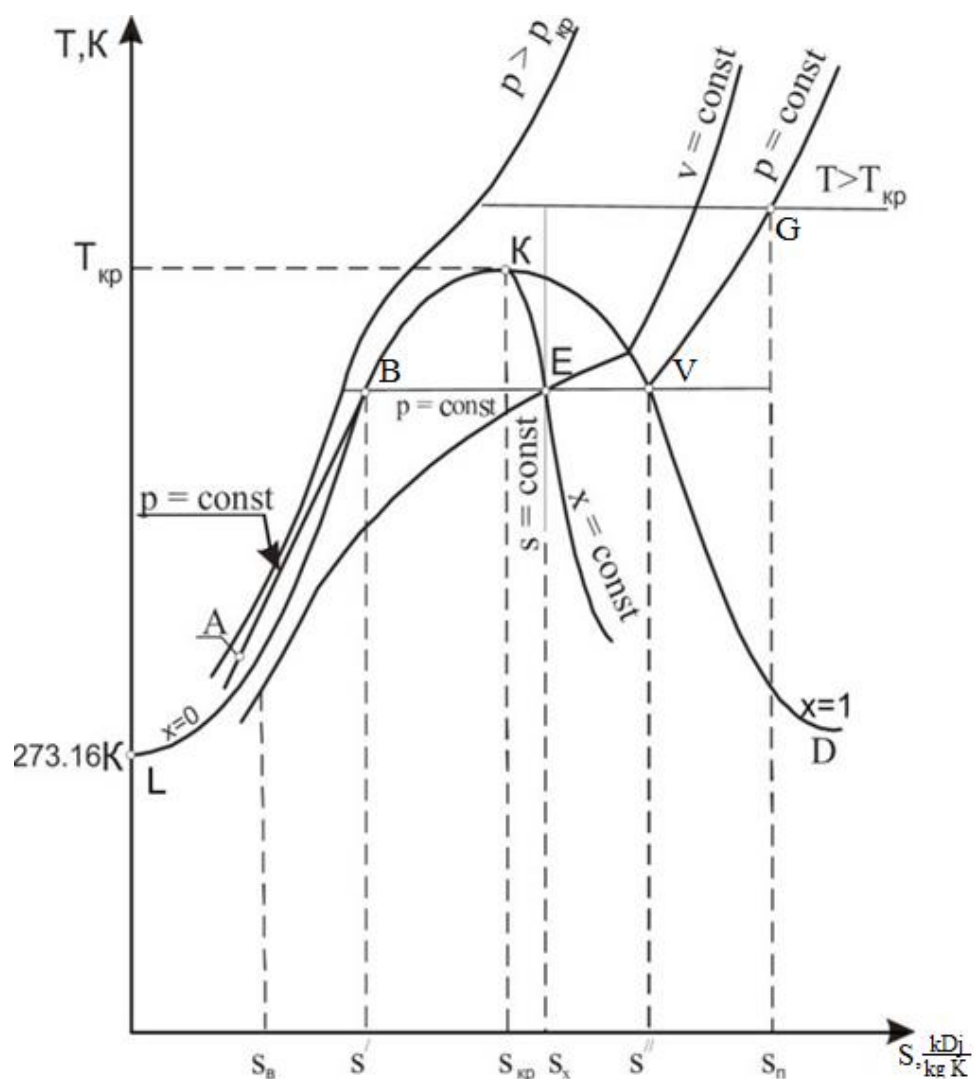
1.7-rasm. Suv bug'ining fazaviy (T, s) – diagrammasi
