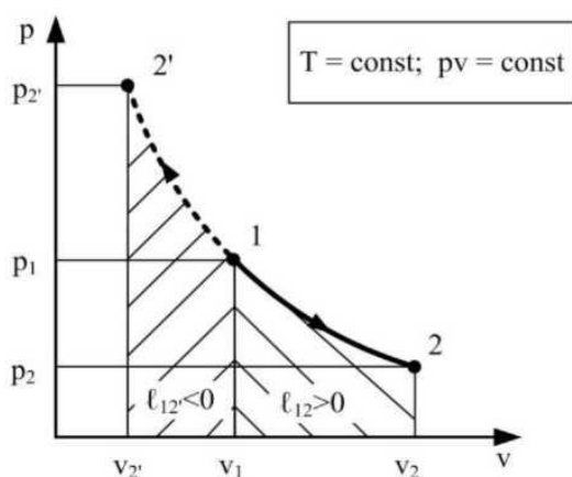
1.3-rasm. Ideal gaz kengayishi va siqilishining izotermik jarayoni
