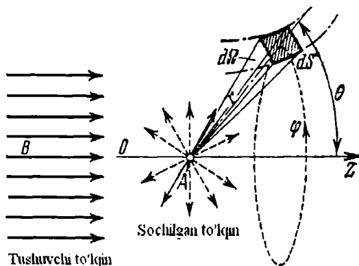
25-rasm. Kvant mexanikasida zarrachalarning to'qnashishi.
