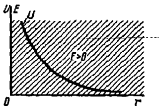
14-rasm. Itarish holati uchun potensial energiya ko'rinishi.
