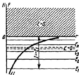
15-rasm. Markazga tortishish holati uchun potensial energiya ko'rinishi.
