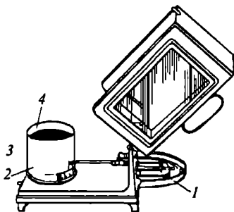
2.8-rasm. Termograf.
