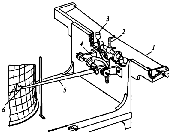
3.7-rasm. Gigrograf.
