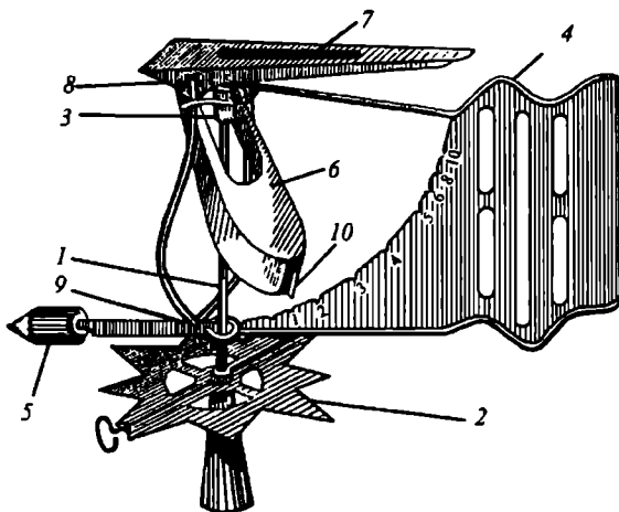
5.1-rasm. Tretyakov shamolo'chagichi.
