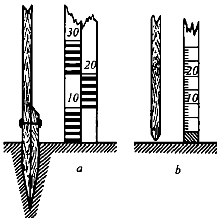
7.4-rasm. Qor o'lhagich reykalari: a – doimiy; b – ko'chma.
