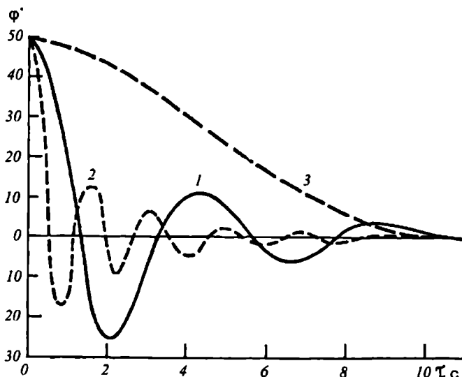
5.5-rasm. Shamol yo'nalishi datchiklarining o'zgaras havo oqimidagi harakatlanish xarakteri. 1 – flyugarka, 2 – bifyugarka, 3 – vindroza.
