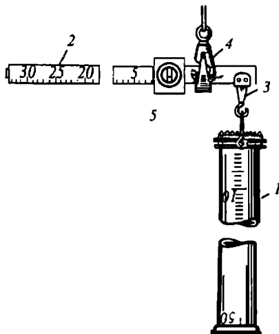
7.5-rasm. Tarozi qor o‘lchagich.
