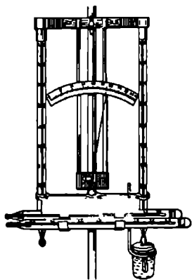
2.1-rasm. Termometrlarning psixrometrik budkaning ichiga o'rnatilishi.
