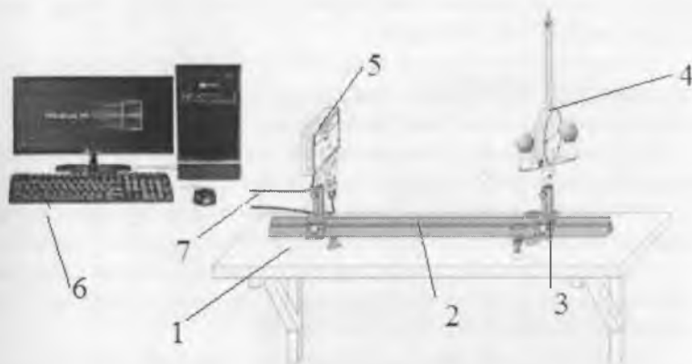
4-rasm. Tajriba qurilmasi: Tebranishni IQ harakat detektori elektron tarzda qayd qiluvchi gravitatsion torsion balansir qurilmasining stoldagi yig'masi. Stol (1), optik rels (2), taglik sterjen (3), gravitatsion torsion balansir (4), IQ holat detektori (5), kompyuter (6), ulovchi kabellar (7).
