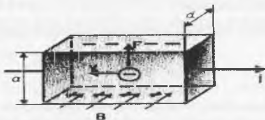
3- rasm. Magnit maydonida zaryadlangan zarra
