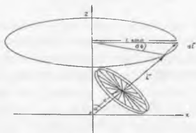
1-rasm. Giroskop pressesiyasi
