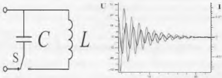
1-rasm: Kalitli tebranish konturi. 2-rasm: Kuchlanish va tok tebranishlari.
