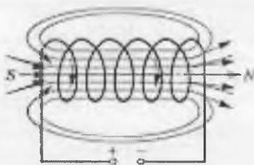
1 - Rasm. Solenoid
