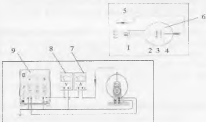
3-rasm. Diodning xarakteristikasini o'lchash uchun eksperimental qurilma. qizdiruvchi vilka(1), katod plastinkasi(2), katod qizdirgich simi(3), anod(4), anodni ulash simi(5), havosi so'rib olingan shisha bolon(6), ampermetr(7), voltmeter(8), tok manbai(9).
