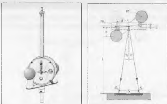
3-rasm. Kavendishning gravitatsion torsion balansir (chapda) va tajriba qurilmasining tuzilish chizmasi (o'ngda)
