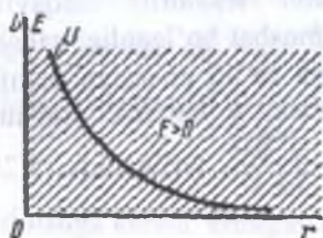
14-rasm. Itarishish holati uchun potensial energiya ko'rinishi.
