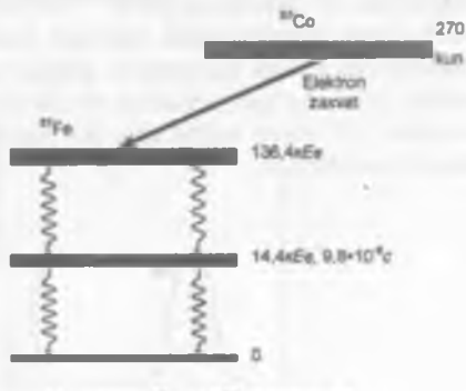
23.11-rasm. ^{57}\text{Co} \rightarrow ^{57}\text{Fe} yemirilish chizmasi.
