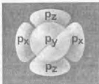
25.3-rasm. Azot atomining 3 ta 2r elektroni (r, orbita-ning 2-pallasi rasmda ko'rsatilmagan).
