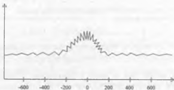
29.25-rasm. Djozefsonning ikkita tunnel o'tishi parallel ulanganda magnit maydonga bog'liq bo'lgan tokning o'zgarish grafigi.
