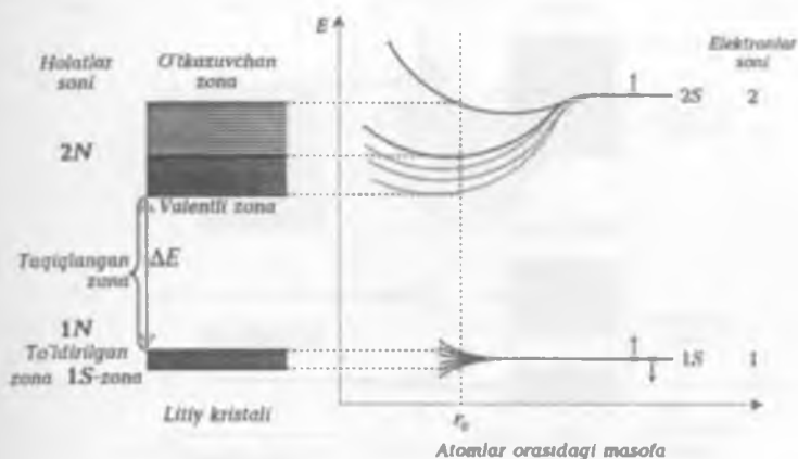
27.6-rasm. Litiy kristalli uchun energetik zonalar. r_0 - kristall dolmiysi
