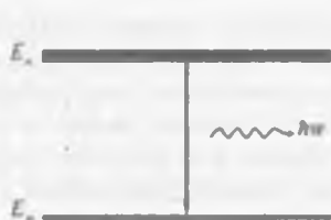
23.4-rasm. E_n dan E_m ga o'tish.
