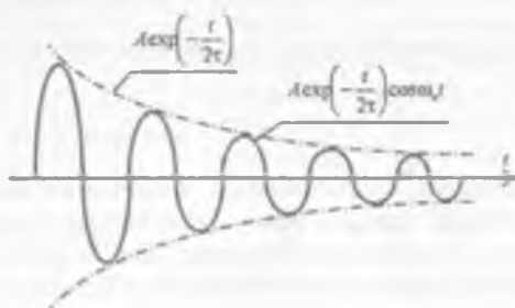
21.1-pasm. Ekspontensial so'nuvchi tebranish jarayon deyarli davriy bo'lib, tebranish chastotasi taxminan \omega_0 ga teng.
