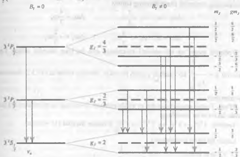
19.4-pach. Atom sathlarining kuchsiz magnit maydonda Zeyeman anomal ajralishi
