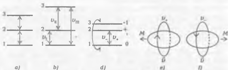
32.10-rasm. Ko'p sathli sistemalar dinamikasi
