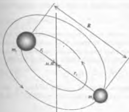
24.7-rasm. Ikki atomli molekulaning massa markazini topish.
