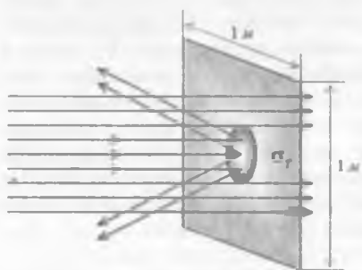
20.6-pasm. Sochilishning Tomson kesimi ( \sigma_T )
