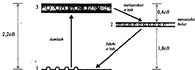
22.5-rasm. 3 sathli lazerning energetik chizmasi (yoqut misolida).
