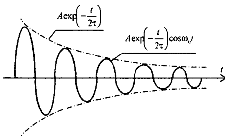
21.1-rasm. Eksponensial so'nuvchi tebranish jarayon deyarli davriy bo'lib, tebranish chastotasi taxminan \omega_0 ga teng.
