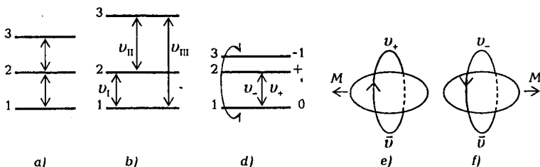
32.10-rasm. Ko'p sathli sistemalar dinamikasi
