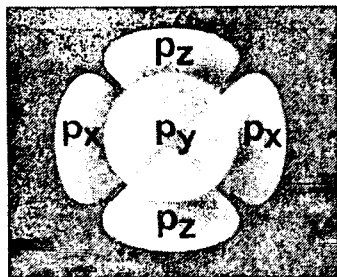
25.3-rasm. Azot atomining 3 ta 2r elektroni ( r_p orbitalning 2-pallasi rasmda ko'rsatilmagan).
