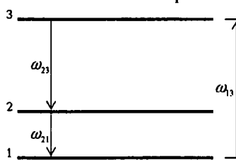
32.9-rasm. Uch sathli sistema.
