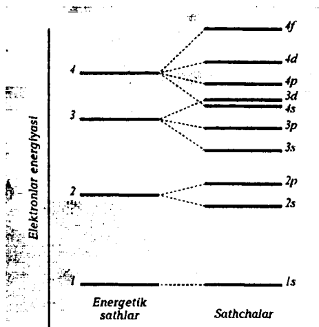
26.4-rasm. Energetik sathlar va sathchalar
