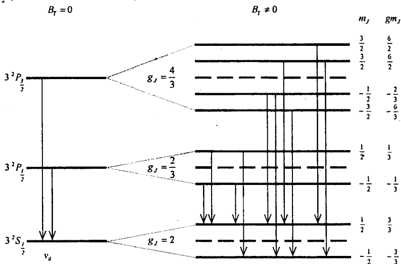
19.4-рasm. Atom sathlarining kuchsiz magnit maydonda Zeyeman anomal ajralishi
