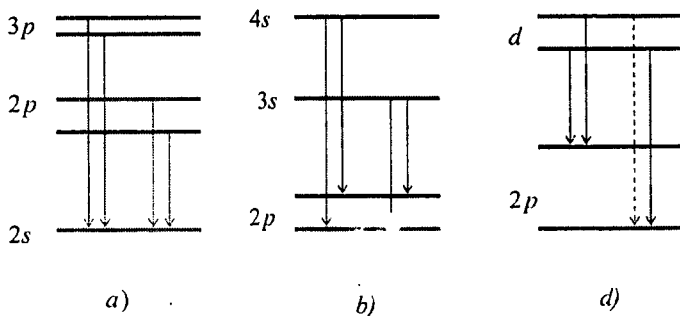
18.10-rasm. a) - p sathlardan 2s sathga o'tish chizmasi; b) - s sathlardan 2p sathga o'tish chizmasi; d) - d sathlardan 2p sathga o'tish chizmasi;
