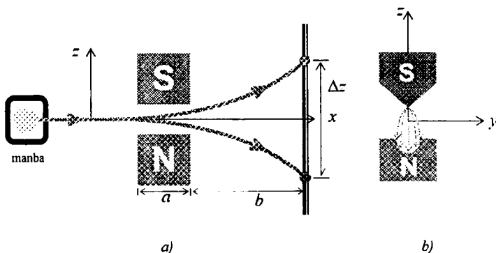
18.6-rasm. a) Shtern-Gerlax tajribasi; b) nojins magnetmaydonning hosil bo'lishi
